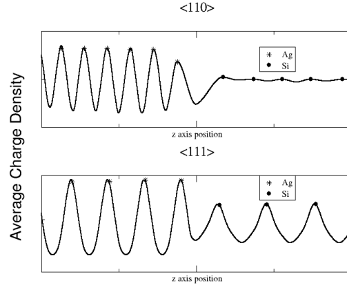
FIG. 6. Averaged, normalized charge densities along the 001 axis of the 110//110 (a) and 111//111 (b) interfaces. The positions of the atomic layers are indicated by a point.
