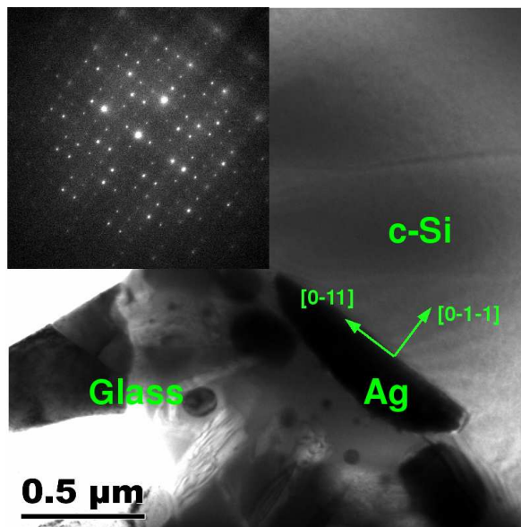
FIG. 2. Bright field TEM image and diffraction pattern of a Ag crystallite (dark contrast area) embedded in the c-Si matrix (area to the right).
