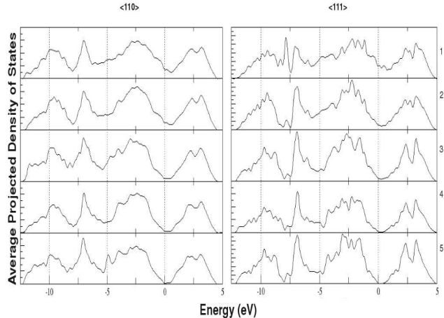
FIG. 7. Averaged projected density of states of the Si atoms in each layer moving away from the Si/Ag interface from the top down. The supercell Fermi level is set to zero.
