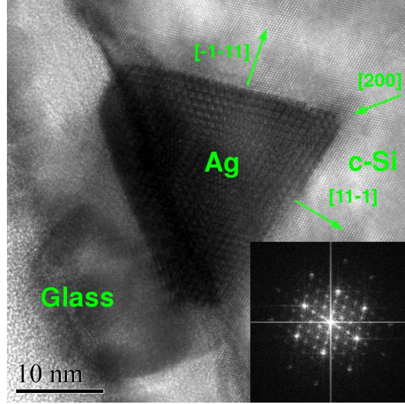
FIG. 3. High resolution TEM image of a Ag crystallite (triangular feature) embedded in the c-Si matrix (area to the right). The inset shows the Fourier transform of the Ag crystallite plus Si matrix.
