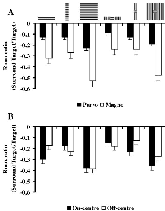
Fig. 4. R_{\max} ratio [ (R_{\max} with extraclassical stimulation - R_{\max} with receptive-field stimulation alone)/ R_{\max} with receptive-field stimulation alone] in parvocellular and magnocellular neurons, and on-center and off-center neurons with V1 intact. The R_{\max} ratio of magnocellular neurons was reduced to a greater degree than that of parvocellular neurons by extraclassical stimulation (A). There were no differences between on-center and off-center cells in the degree of reduction of the R_{\max} ratio by extraclassical stimuli (B).
