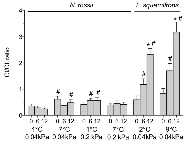
Figure 5. CI/CII ratio in liver mitochondria from warm/hypercapnia acclimated N. rossii and L. squamifrons . N. rossii acclimated to 1°C, 0.04 kPa CO 2 (control), n=9; 7°C, 0.04 kPa CO 2 (warm normocapnic), n=5; 1°C, 0.2 kPa CO 2 (cold hypercapnic), n=10; and 7°C 0.2 kPa CO 2 (warm hypercapnic), n=10, and in mitochondria from control (2°C, 0.04 kPa CO 2 , n=7) and warm acclimated (9°C, 0.04 kPa CO 2 , n=5) L. squamifrons . * indicate a significantly elevated CI/CII ratio compared to the 0°C assay within an control/acclimation group (ANOVA, P<0.05). # indicate significantly elevated CI/CII ratios compared to the control group at the respective assay temperature (ANOVA, P<0.05). Values are given as means ± SEM. doi:10.1371/journal.pone.0068865.g005
