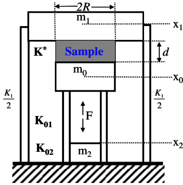
Figure 1: Mechanical Model of the PAV
