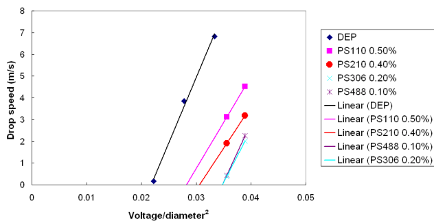
Figure 5: MicroFab nozzle jetting viscoelastic fluids. The PS series, chosen to have similar linear viscoelasticity and viscosity, have similar jetting thresholds [12]; the solvent DEP has a somewhat lower jetting threshold.
