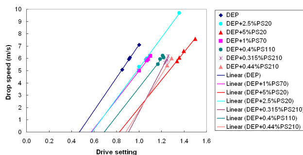
Figure 3: Xaar XJ126-200 nozzle jetting dilute PS+DEP (polystyrene) fluids.
