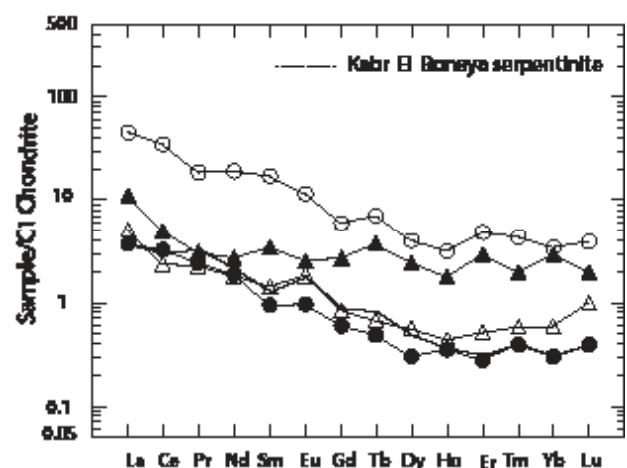
FIGURE 8 | Chondrite normalized REE plots for the averages of listwaenites and serpentinites. Chondrite normalization values are from Sun and McDonough (1989). Symbols as in Figure 6.
