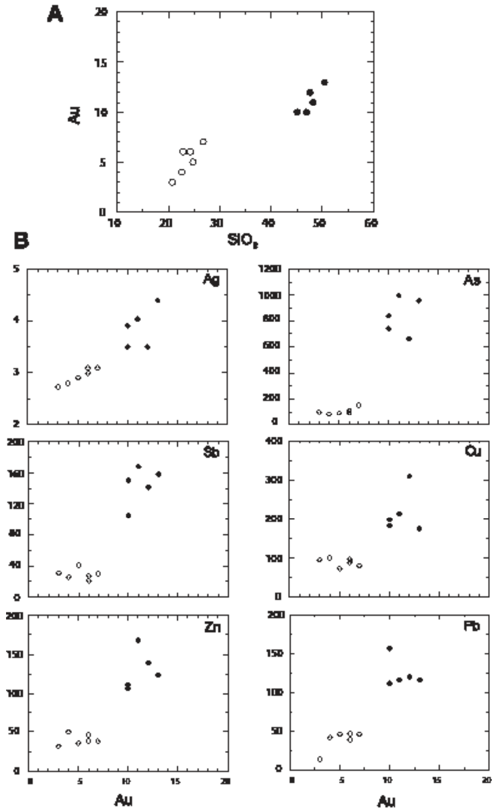
FIGURE 7 | A) Correlation of SiO 2 with Au in the studied listwaenites, B) Correlations of Au element with Ag, As, Sb, Cu, Zn and Pb in the studied listwaenites. Symbols as in Figure 6.
