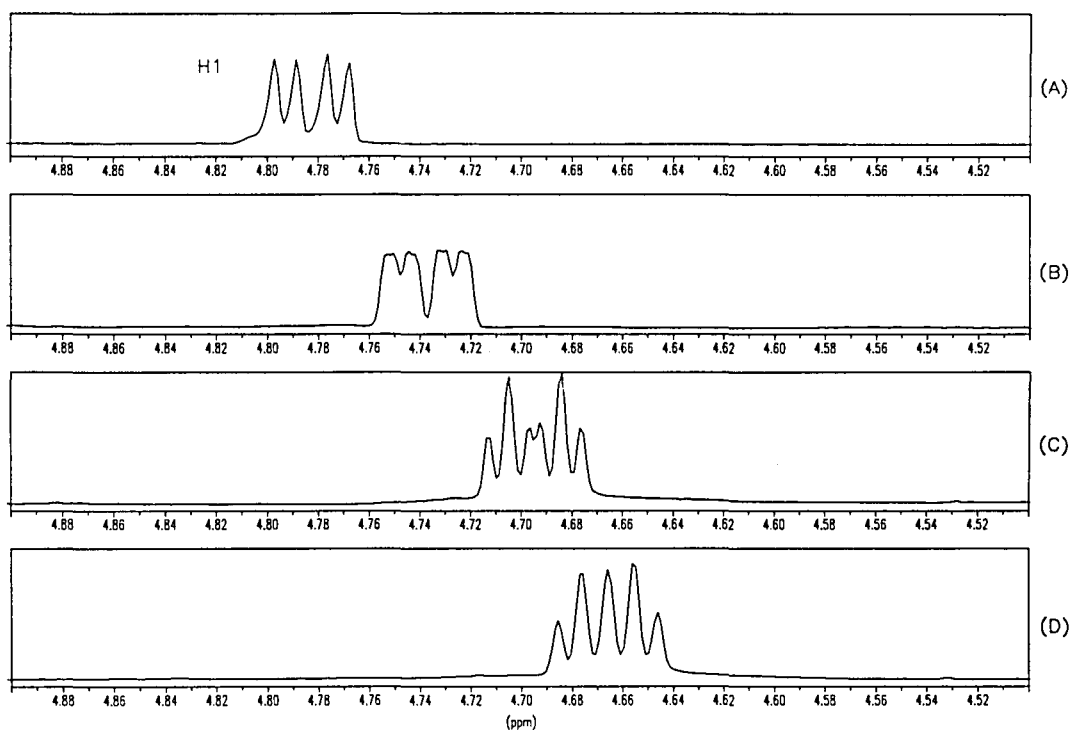
Espectre 11-14a
