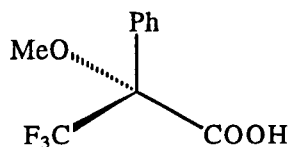
Figura 2-2 : ( R )- MTPA
