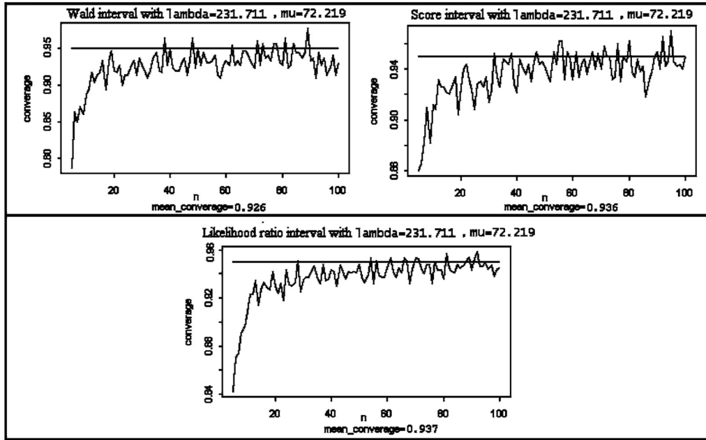
Figure 1: Coverage probability with fixed parameters ( \lambda, \mu ) and variable n from 5 to 100.
