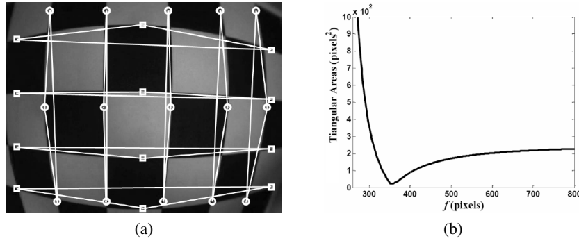
Figure 4: Estimation of f ; (a) triangles; and (b) triangular areas for a range of value of f .
