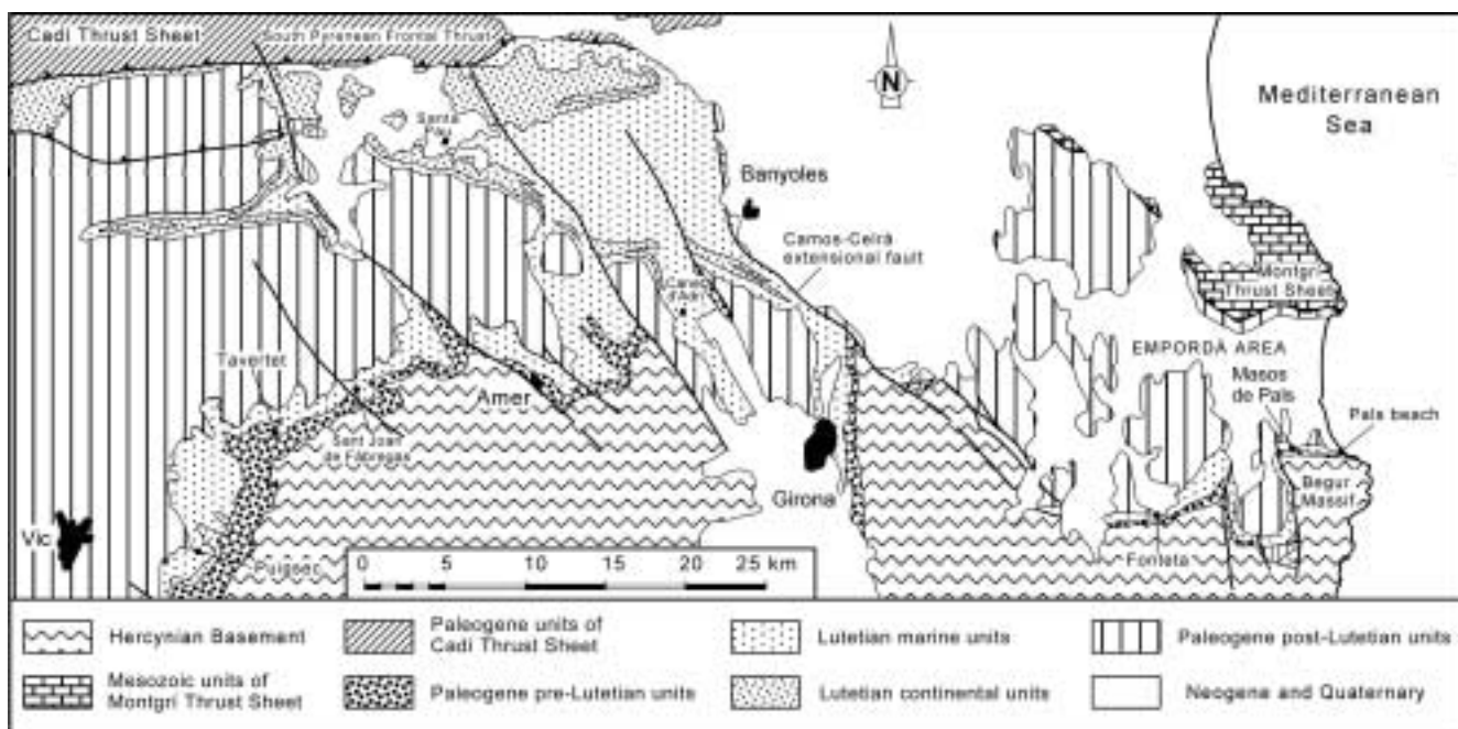
FIGURE 4 | Geological sketch of the Amer-Vic and Empordà area.
