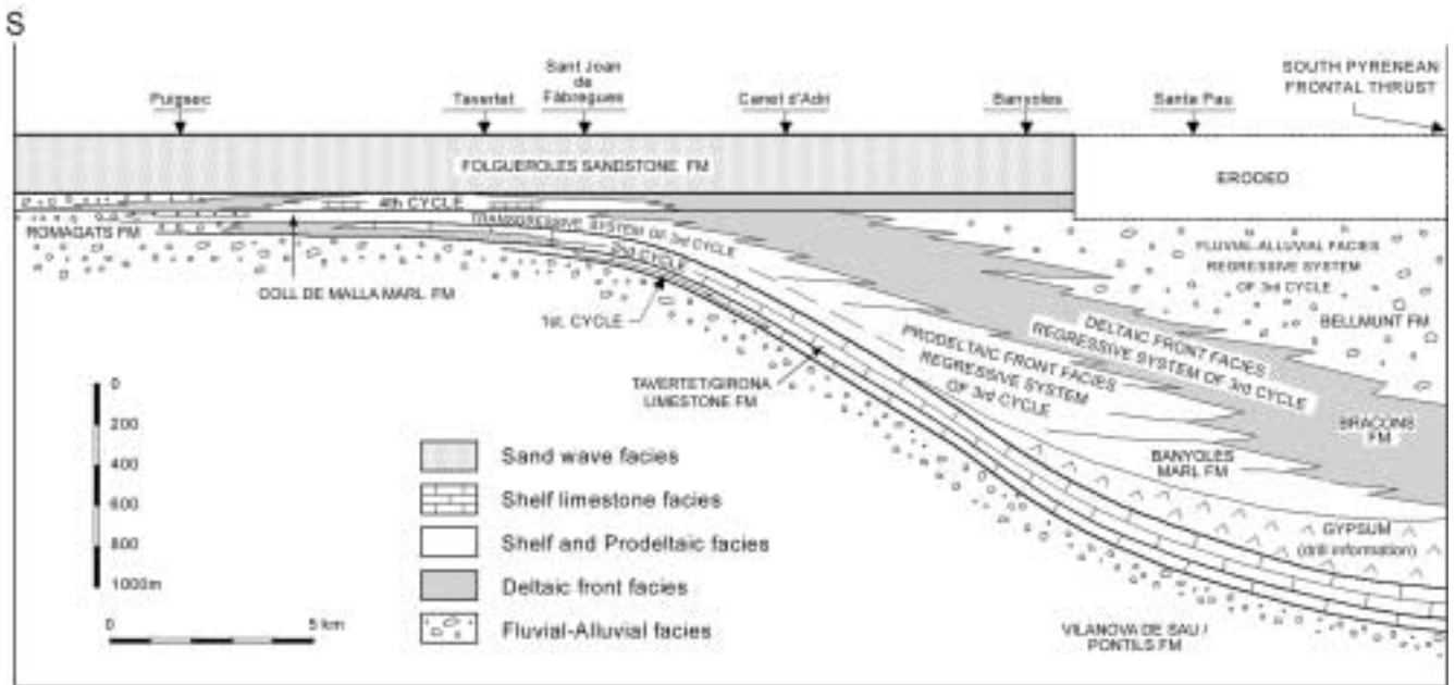
FIGURE 5 | Stratigraphical sketch across a north-south section showing the evolution of the facies during the Lutetian cycles.
