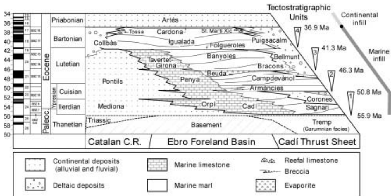
FIGURE 3 | Stratigraphic panel across the Ebro Foreland Basin between the Cadí Thrust Sheet and the Catalan Coastal Ranges, modified from Vergés et al. (1998). Biostratigraphic data combined with magnetostratigraphic information (Burbank et al. 1992a,b; Vergés and Burbank 1996; Serra-Kiel et al. 1994) define the chronostratigraphic framework of this area. Global polarity time scale from Cande and Kent (1995). Larger foraminifers biozones (SBZ) from Serra-Kiel et al. (1998a, b).
