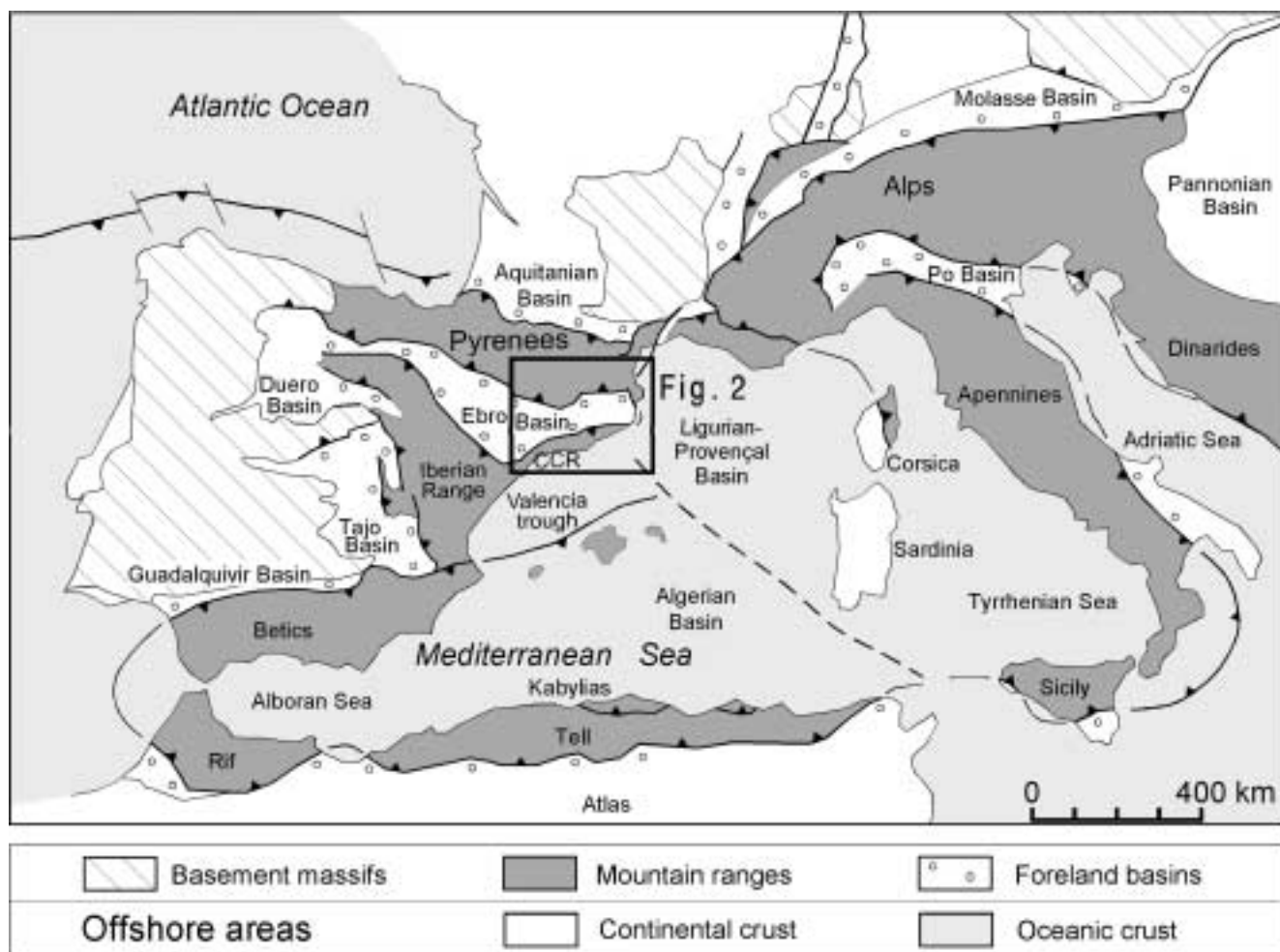
FIGURE 1 | Tectonic sketch of the Western Mediterranean showing the location of the Tertiary orogenic belts and adjacent foreland basins according to Vergés et al. (1998). Thick black lines with black triangles bound shaded orogenic regions. C. C. R.= Catalan Coastal Ranges.
