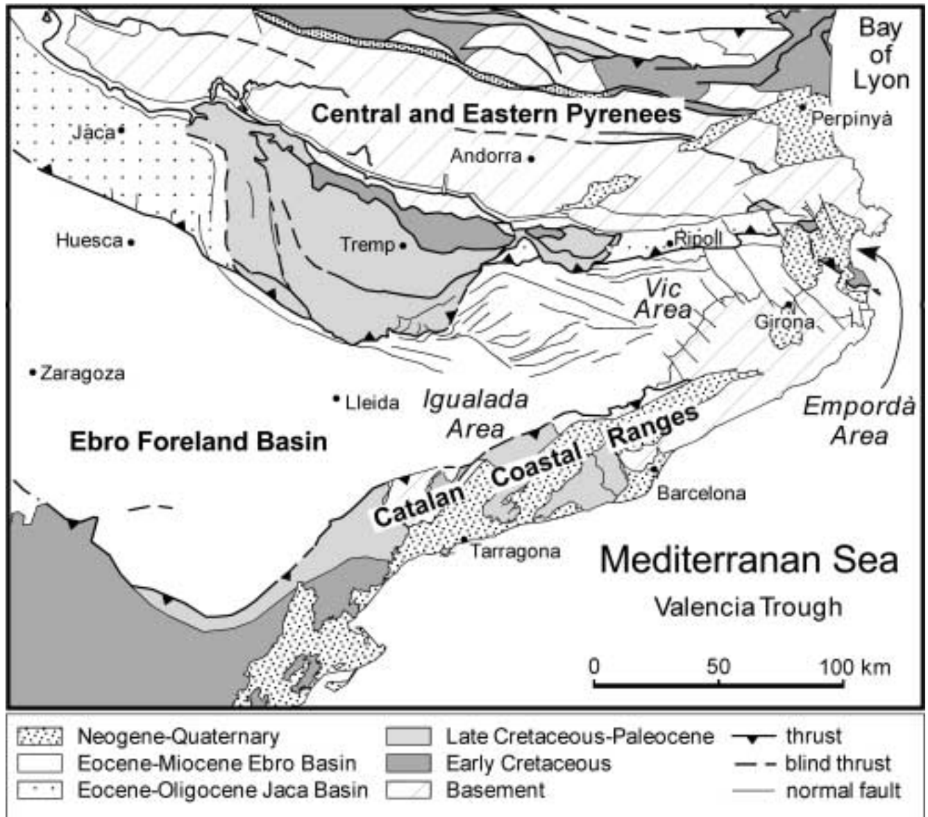
FIGURE 2 | Geological sketch of the eastern part of the Ebro Foreland Basin between the Pyrenean thrust belt to the north and the Catalan Coastal Ranges to the south according to Vergés et al. (1998).
