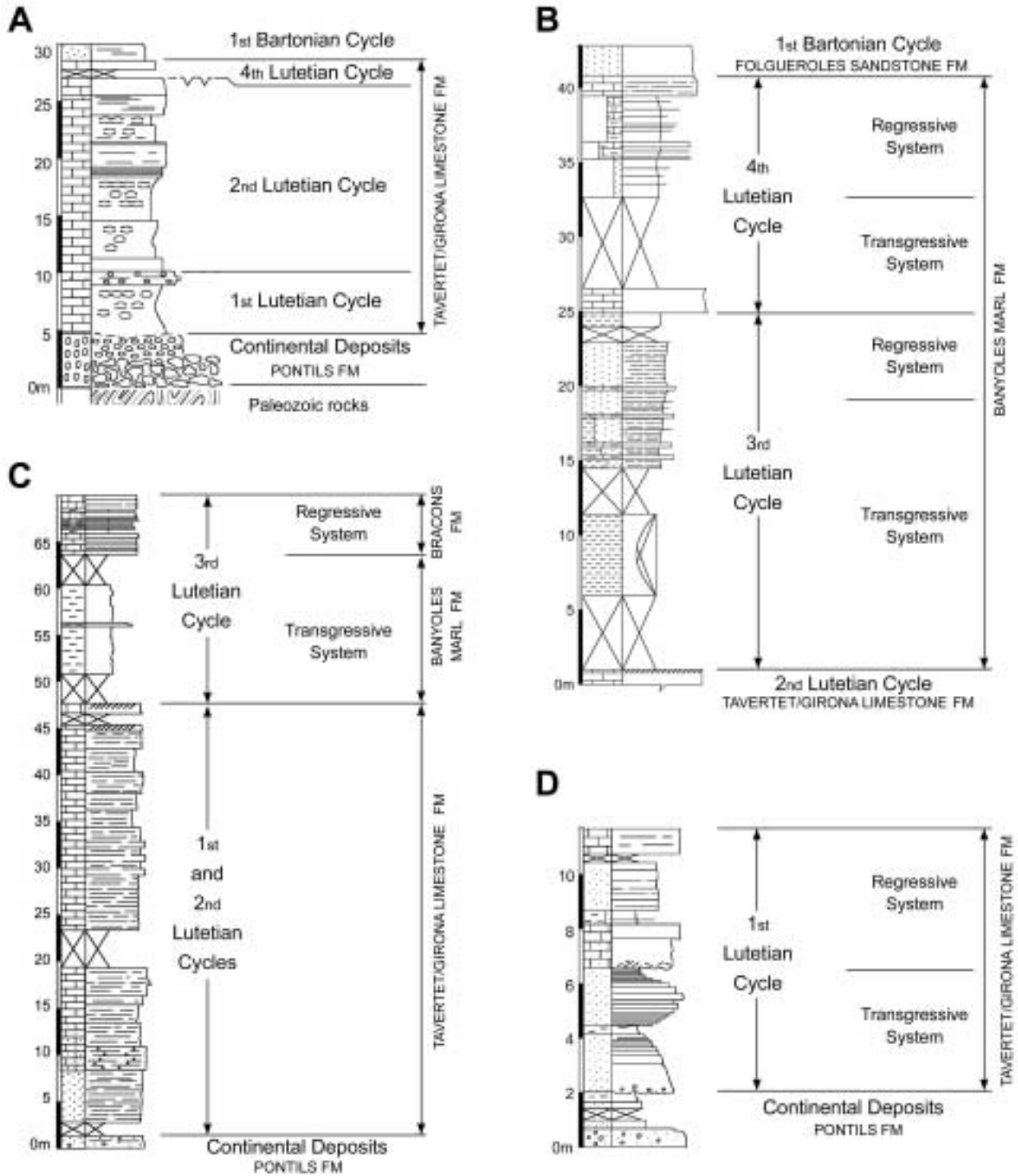
FIGURE 7 | Selected stratigraphic sections showing the Lutetian sedimentary cycles in the Empordà area (Fig. 6). A: Pals beach section, B: Massos de Pals section, C: Fonteta (Can Ametller) section, D: Fonteta (Can Barrabàs) section.
