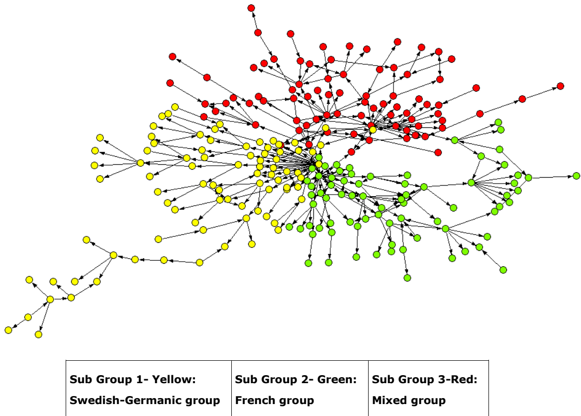
Figure 1. Subsets from the Girvan-Newman algorithm applied on the largest weak component 6 .
