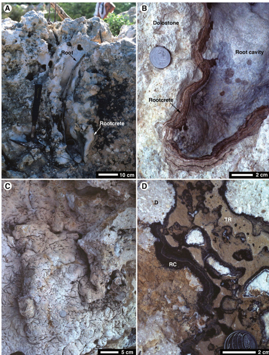
FIGURE 2 | Field photographs of root calcretes in the Cayman Formation, northeast part of Grand Cayman. A) Root calcrete surrounding tree roots in dolostones in upper part of Cayman Formation. B) Brown, thinly laminated root calcrete lining cavity created by tree roots. C) Cavity facing surface of root calcrete showing small grooves that were once filled by tree rootlets and root hairs. D) Root cavity in dolostone lined with manganese-rich root calcrete (RC) and filled with lithified terra rossa (TR).
