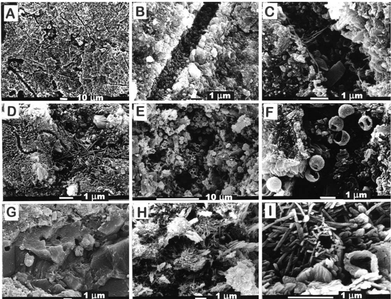
FIGURE 6 | SEM images. A) Microborings showing a very homogeneous distribution along the calcrete, in this case micritic microfabric. B) Straight microboring outlined by coarse calcite crystals. C) Microboring showing a partial infill of calcite needles and euhedral calcite crystals. D) Needle calcite crystals of different sizes they are associated with curved microborings. E) Spores occurring in the porosity of the alveolar septal structures. F) Detailed view of the spores, they tend to occur in groups. G) Spores in the coarser calcite crystals. H) Messes of needles giving places to the formation of irregular bodies of 1-2 µm size. I) Needles on organic structure either filaments or spores.
