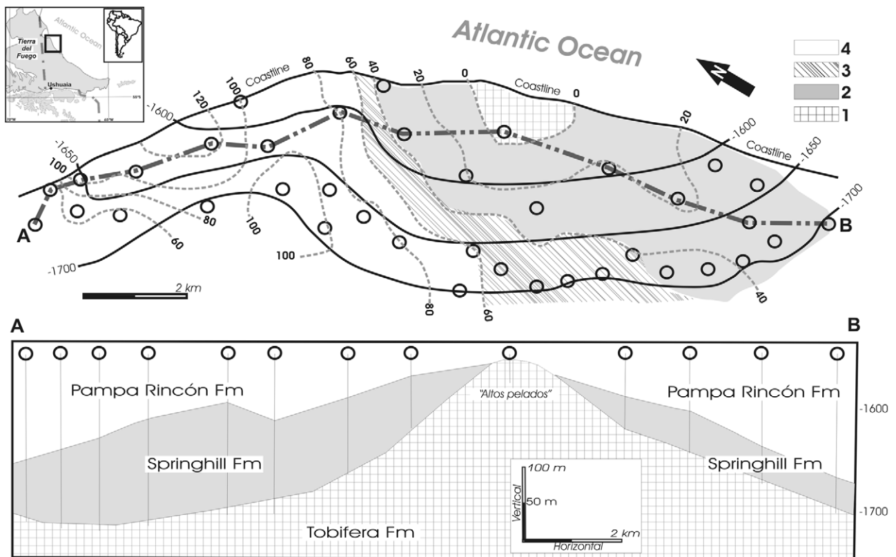
FIGURE 11 | Onshore San Sebastián oil field characteristics (see location in Figure 10). Isopach and contour map of the top of the Springhill Fm and A-B cross section showing the productive structure (circles: production wells). Springhill Fm deposits: 1: missing; 2: continental; 3: transitional; and 4: marine and continental. Continuous line: structure contour on top of Springhill Fm (depth in meters below sea level). Discontinuous lines: isopach of total Springhill Fm (thickness shown in meters).
