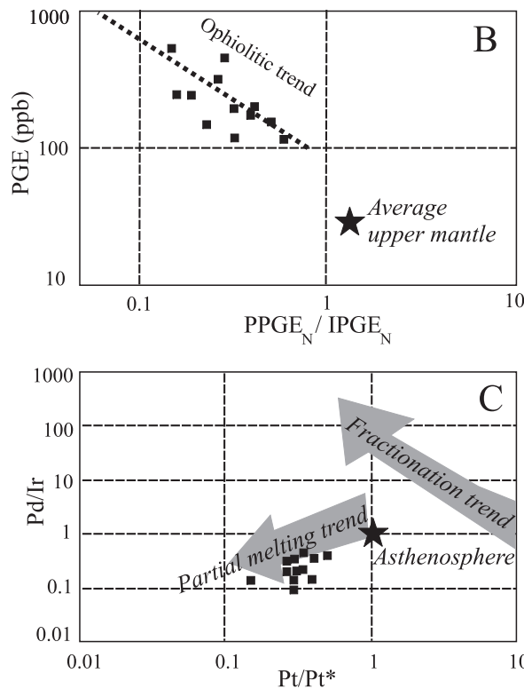
FIGURE 5 | A) Chondrite-C1 (Naldrett, 1981) normalized PGE patterns of the Eskişehir chromitites and comparison with the chromitites hosted in the ophiolitic mantle (grey field). Data from: Proenza et al. (1999); Economou-Eliopoulos (1996); McEluff and Stumpfl (1990); Gauthier et al. (1990); Kojonen et al. (2003); Büchl et al. (2004); Uysal et al. (2005); B) Chondrite-normalized PPGE/IPGE vs PGE for the Eskişehir chromitites. Chondrite and average upper mantle values are from Leblanc (1991) and ophiolitic trend is from Melcher et al. (1999); C) Plot of Pt/Pt* [Pt N /(Rh N *Pd N ) 1/2 ] vs Pd/Ir of the Eskişehir chromitites. Fractionation and partial melting trends are from Garuti et al. (1997).
