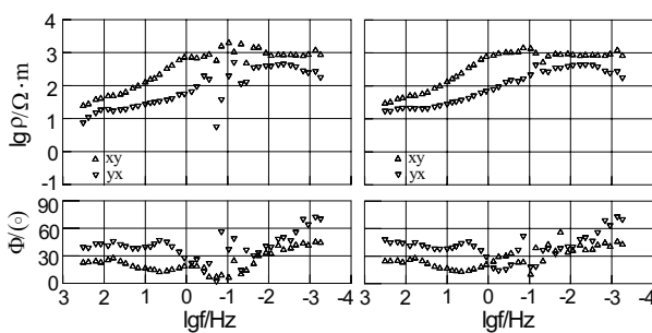
FIGURE 2 | Comparison of analysis results for site 71 using the remote reference MT method (RR). Left charts show apparent resistivity and impedance phase without using RR. Right charts show those using RR. Upper charts are apparent resistivities, where ordinates are resistivity ( \Omega \cdot m ) in logarithmic scale. Lower charts are impedance phases, where ordinates are degrees. Abscissas are frequencies (Hz). xy and yx denote the data (apparent resistivity and impedance phase) for the electrical field components, perpendicular and parallel to the line direction (TE and TM polarizations), respectively.
