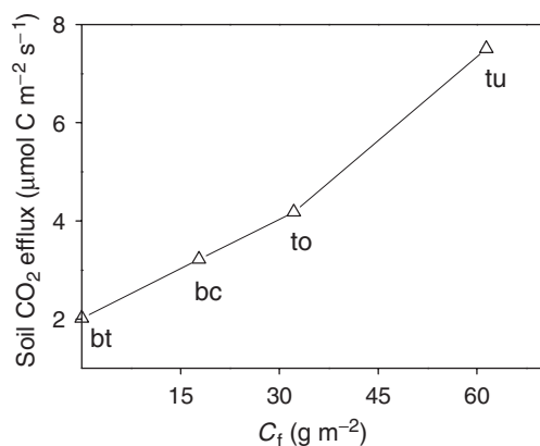
Fig. 5 Measured decomposition-derived CO_2 effluxes at time 0 and 20\ ^\circ C vs. initial C_f quantity calculated with Eqn (7).
