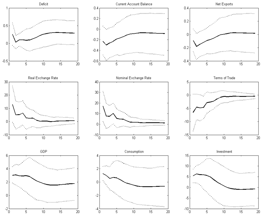
Figure 3: Robustness: impulse response functions to a government spending shock.
