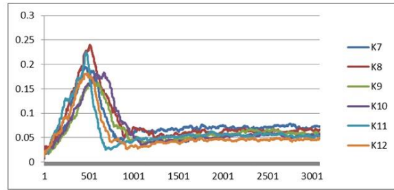
Fig.13. Different crowd panic value with different distribution of KI at the density of 4 persons/m 2
