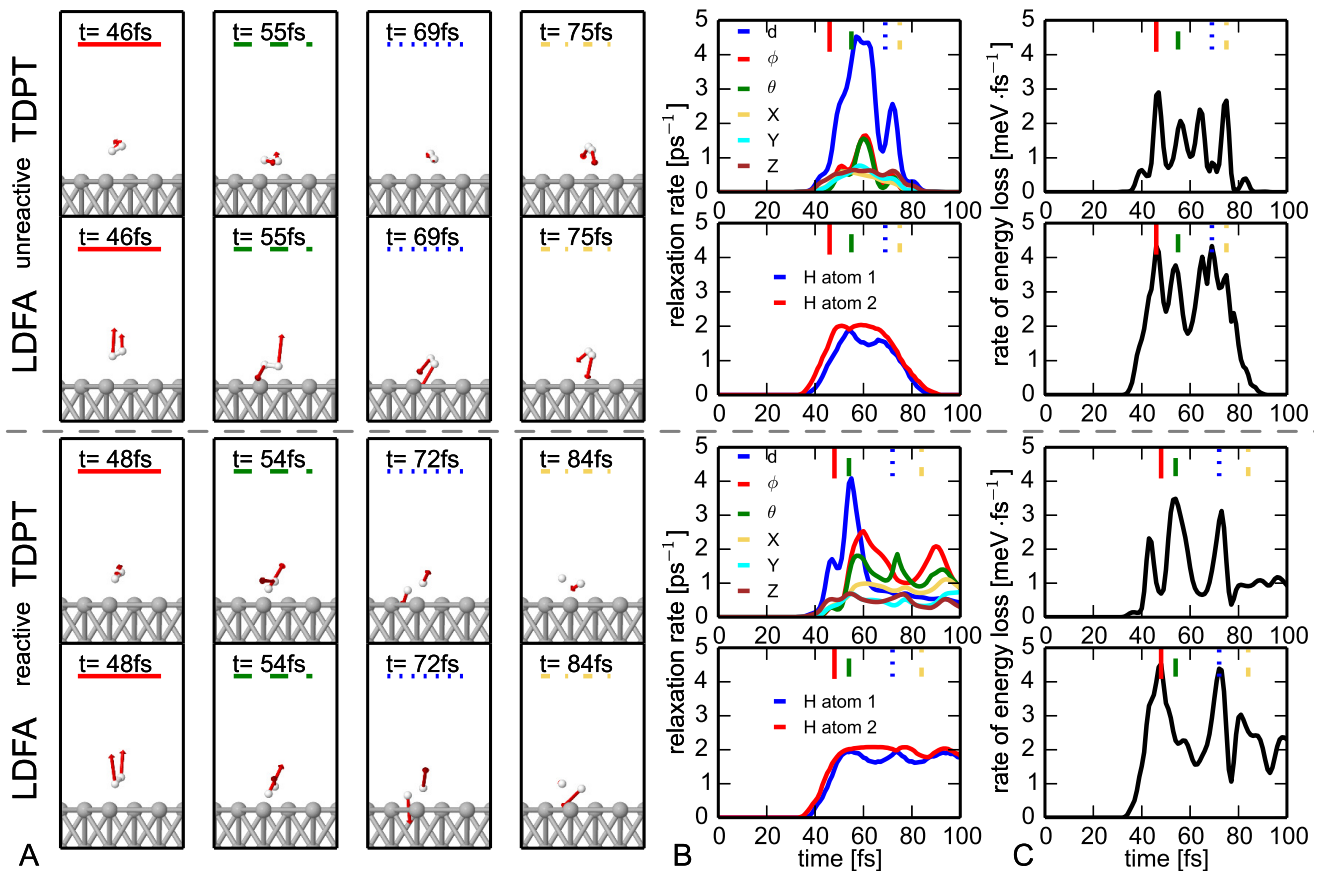
FIG. 2. (A) Snapshots at different times for an unreactive (top) and a reactive (bottom) trajectory. The incidence energy is 1.8 eV. Red arrows indicate the frictional force according to the second term in eq. 1. (B) Relaxation rate in \text{ps}^{-1} projected along the internal coordinates defined in Fig. 1(C). (C) Rate of energy loss in \text{meV}\cdot\text{fs}^{-1} along the trajectory. Vertical lines indicate the snapshots in time shown in panel A.
