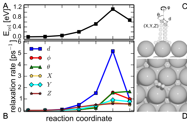
FIG. 1. (A) Relative energy along a minimum energy path (MEP) of \text{H}_2 dissociation on Ag(111). (B) Nonadiabatic relaxation rates in \text{ps}^{-1} obtained from the diagonal elements of electronic friction tensor in internal coordinates: bond stretch d , azimuthal angle ( \phi ), polar angle ( \theta ), and the three Cartesian center of mass coordinates of the Hydrogen molecule ( X, Y, Z ). Off-diagonal elements (not shown) can modify relaxation rates by 30% or more. (C) Side view of the dissociation along the minimum energy path. (D) Top view of start and end point of MEP.
