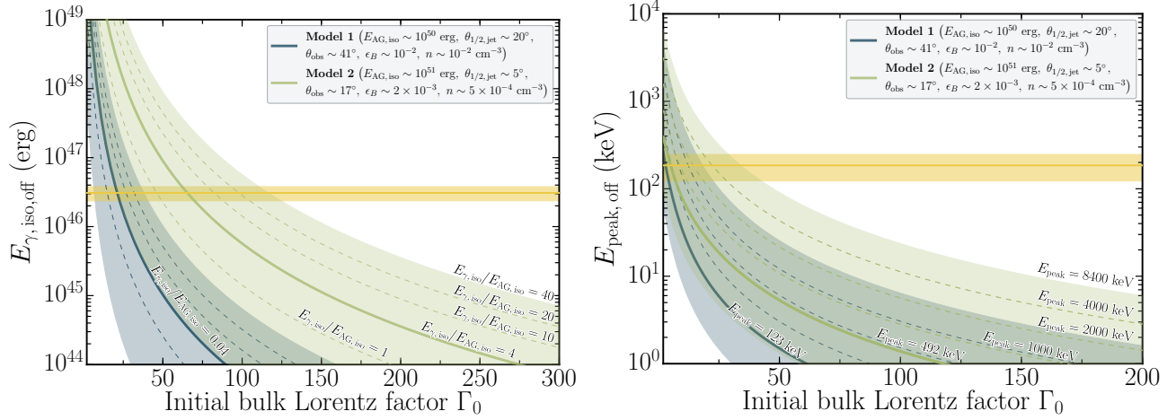
Figure 4. The isotropic \gamma -ray energy release E_{\gamma,\text{iso,off}} and the E_{\text{peak}} of the prompt emission measured by an off-axis observer, as a function of \Gamma_0 . We use the model in Donaghy (2006) to predict the allowed loci of the parameter spaces for GRB 170817A. The loci depend on the jet geometry and the viewing angle which we obtained from the broadband modeling in §3.2. The known distributions for E_{\gamma,\text{iso}}/E_{\text{AG,iso}} ( Cenko et al. 2011 ) as well as the observed peak energy distribution of our SGRB comparison sample further limit the possible parameter space to the shaded regions ( Model 1 : blue; Model 2 : red). Curves of particular values are displayed by the dashed curves. The solid curves indicate the location of the distribution mean values. The parameter space is furthermore limited by the results from Fermi reported in Goldstein et al. (2017b) , displayed in yellow. The bands encompassing the Fermi measurements indicate the 1\sigma confidence intervals. These constraints limit \Gamma_0 to < 15 and < 43 for Model 1 and Model 2 , respectively.
