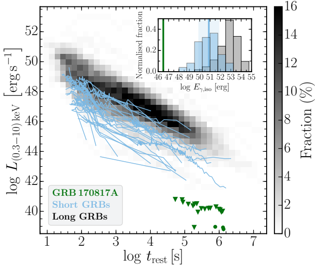
Figure 2. X-ray light curves of GRB afterglows. The parameter space occupied by 402 LGRBs, detected between December 2004 and September 2017, is indicated by the density plot. Light curves of 31 SGRBs with detected X-ray afterglows are shown in light blue. GRB 170817A lies 2.6 orders of magnitude below the other SGRBs. The inset displays the distribution of energy release at \gamma -ray energies (SGRBs: blue; LGRBs: gray). The blue vertical line and shaded region indicate the median value and dispersion of the SGRB distribution, respectively.
