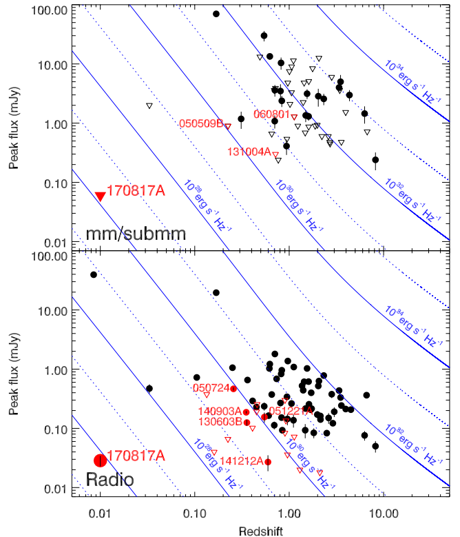
Figure 1. Peak flux densities of GRB afterglows derived from mm/sub-mm (top) and radio (bottom) observations. Filled circles and empty triangles denote detections and 3\sigma limits, respectively. SGRBs are shown in red and LGRBs in black. Solid and dotted blue curves indicate equal afterglow luminosities. The non-detection in the sub-mm corresponds to a luminosity limit of 3 \times 10^{26} \text{ erg s}^{-1} \text{ Hz}^{-1} . The faint radio counterpart detected by Corsi et al. (2017b) suggests a peak luminosity of \sim 7 \times 10^{26} \text{ erg s}^{-1} \text{ Hz}^{-1} .
