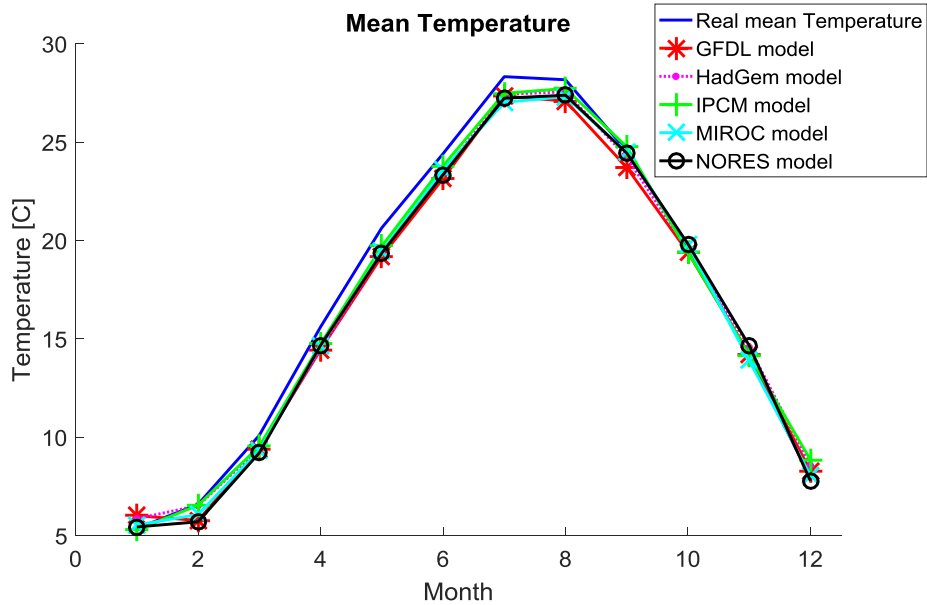
Fig. 4 The real recorded air temperatures (solid line) and those provided by the climate models in the time interval from 1981 to 2005.
