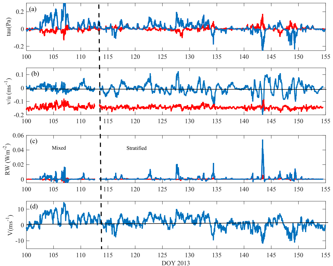
Fig. 3 a Components of surface wind stress: axial (blue) and transverse (red). b Near-surface flow at 3.5-m depth: axial v (blue), transverse u (red) offset by -0.15 \text{ m s}^{-1} . c Components of rate of working RW , axial RW_y (blue), and transverse RW_x (red). d Along-lake wind component V
