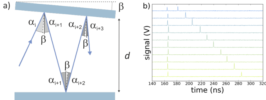
Fig. 2. a) Schematic view of the optical delay line, b) Delay of two consecutive pulses with different central wavelengths measured using a fast photodiode: from top to bottom the angle \beta was reduced to allow four additional reflections for each consecutive measurement.
