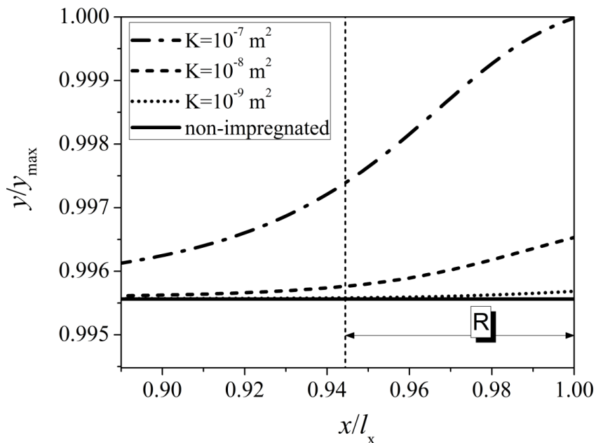
Figure 5-4: Infiltration depth profiles (convergent shapes of line AB) plotted along a 2R distance for three different permeabilities K=10^{-7} , 10^{-8} and 10^{-9} m^2 . For the cases shown here, L_o=2 mm, R=5 mm, V=0.15 m/s and \mu=1000 Pa·s. The horizontal axis is scaled with the l_x length of the computational domain and the vertical distance is scaled with the maximum y_{max} (i.e. y_{max}=l_y+L_o+h_f ) length obtained at x/l_x=1 for K=10^{-7} m^2 . The final
