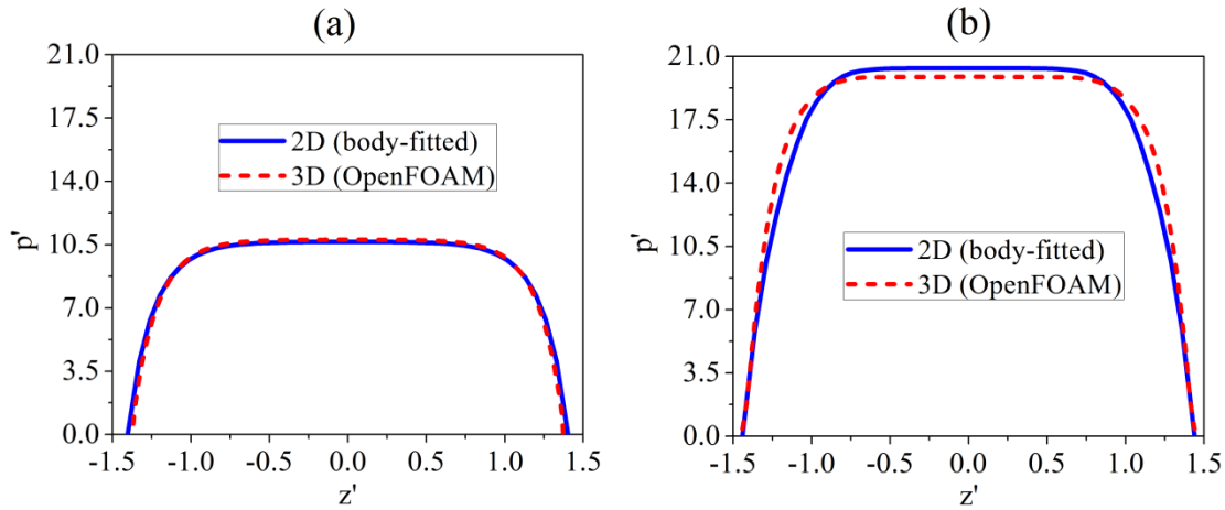
Figure-A.2.2: Pressure distribution in the z -direction at x'=-0.475 for (a) a Newtonian fluid with \mu=5000 \text{ Pa}\cdot\text{s} (2D: 3600 cells, 3D: 8 \times 10^5 cells) and (b) for a shear-thinning fluid with n=0.35 and m=50000 \text{ Pa}\cdot\text{s}^{0.35} (2D: 8100 cells, 3D: 2.4 \times 10^6 cells). Typical process parameters used: V=0.1 \text{ m/s} , R=0.125 \text{ m} , H_o=5 \times 10^{-4} \text{ m} and W_i=0.1 \text{ m} .
