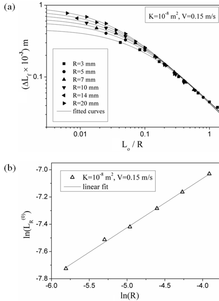
Figure 4-7: (a) Effect of the pin radius R on the impregnation depth \Delta L_f for different values of the dimensionless depth L_o/R ( K=10^{-8} \text{ m}^2 ); and (b) effect of the pin radius R on the impregnation depth L_R^{(0)} in the limit of an initially dry substrate ( L_o \rightarrow 0 ) for K=10^{-8} \text{ m}^2 and \mu=1000 \text{ Pa}\cdot\text{s} .
