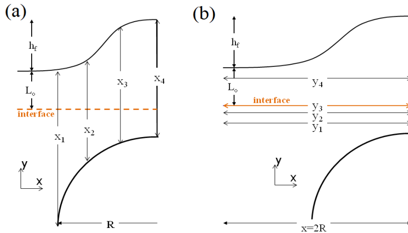
Figure 5-5: Schematic representation of different directions on which the (u_x, u_y) velocity components are plotted (a) corresponds to u_x and (b) for u_y (note: y_I = \delta/2 ). Figure not to scale.
