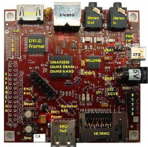
Figure 48 - BeagleBoard C4
