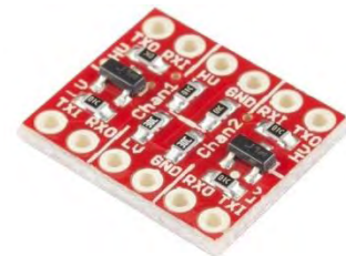
Figure 16 - Logic Level Converter
