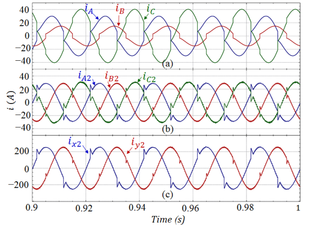
Fig. 9. Simulation results when both sections are loaded: (a) Public grid currents before compensation; (b) Public grid currents after compensation; (c) Currents on the secondary of the V/V transformer after compensation.
