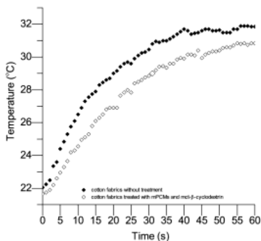
Fig. 6. Time delay to reach 33 °C of untreated cotton and cotton functionalized with mPCM and MCT-β-CD
