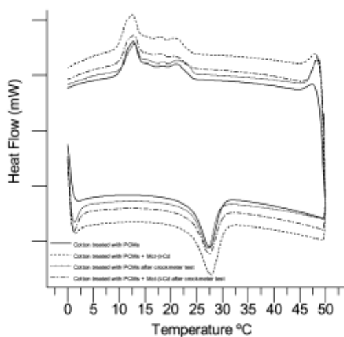
Fig. 5. DSC thermograms of cotton fabrics functionalized with mPCM and conjugated with mPCM and MCT-β-CD before and after rubbing test
