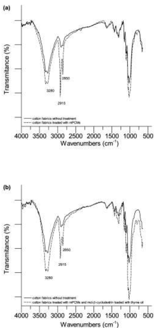
Fig. 3. FTIR spectra of (a) cotton fabrics functionalized with mPCM and (b) cotton fabrics functionalized with mPCM conjugated with MCT- \beta -CD loaded with thyme oil
