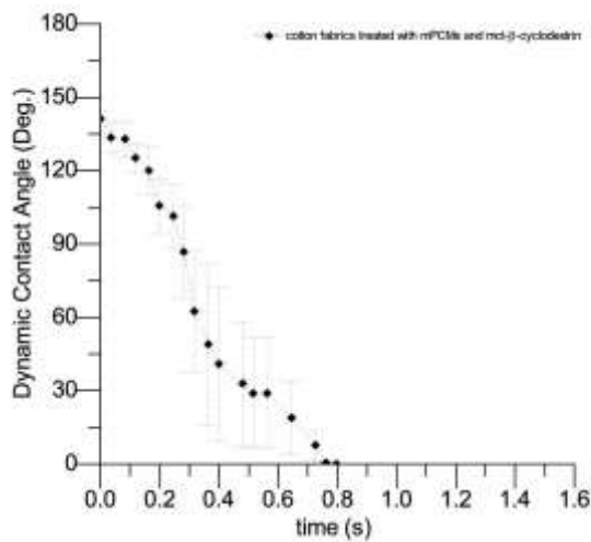
Fig. 8. Dynamic contact angles of the samples
