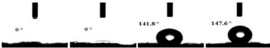
Fig. 7. Static contact angle for tested samples: (a) cotton; (b) cotton with MCT-β-CD; (c) cotton with mPCM; (d) cotton with mPCM and MCT-β-CD
