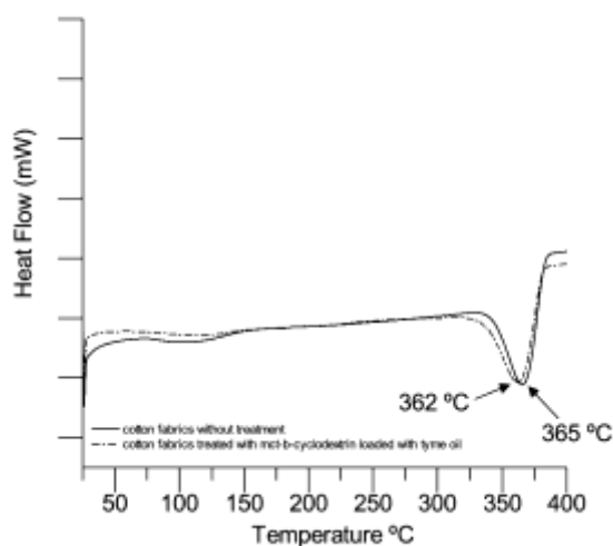
Fig. 4. DSC thermograms of untreated cotton and cotton functionalized with MCT- \beta -CD
