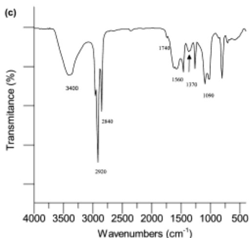
Fig. 1. FTIR spectra of: (a) thyme oil, (b) MCT- \beta -cyclodextrin and (c) mPCMs
