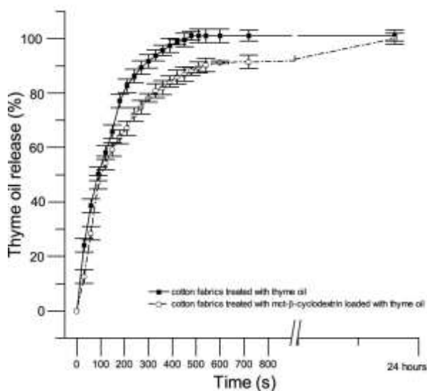
Fig. 11. In vitro controlled release profiles in alkaline solution thyme oil from cotton with thyme oil absorbed and cotton with thyme oil inside MCT- \beta -cyclodextrin
