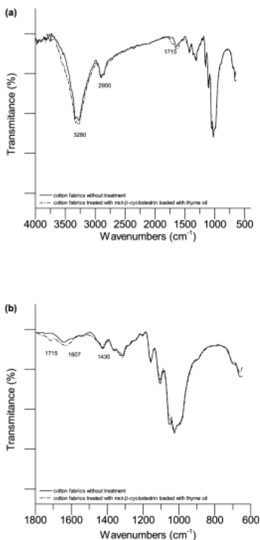
Fig. 2. FTIR spectra of cotton fabrics untreated and functionalized with MCT-β-CD and thyme oil
