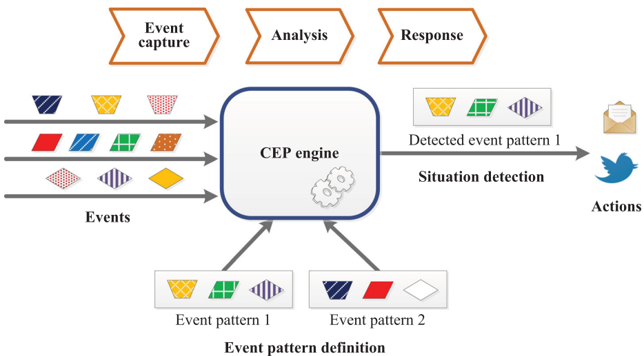
Figure 1. Event pattern recognition in CEP.
