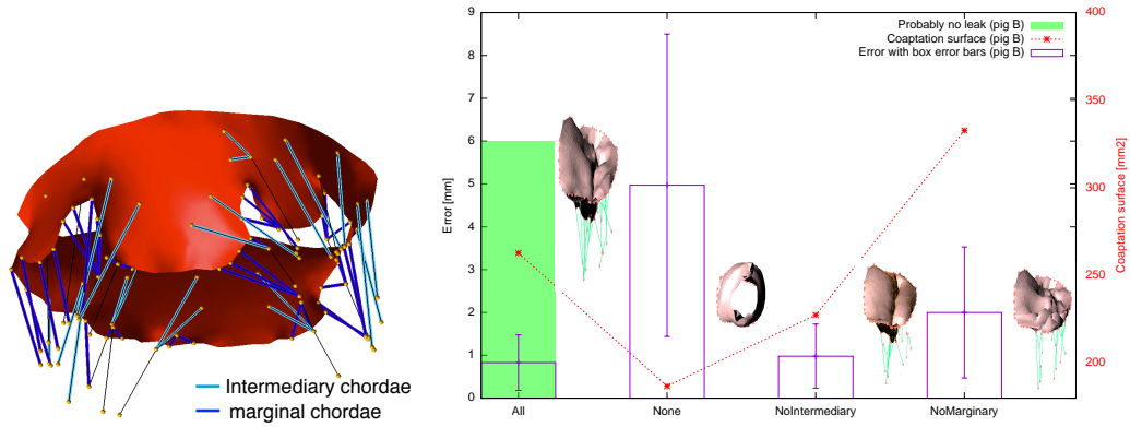
Figure 16. Chordae influence. Left : attachment point labeling, right : Metric plots based on different chordae configurations.
