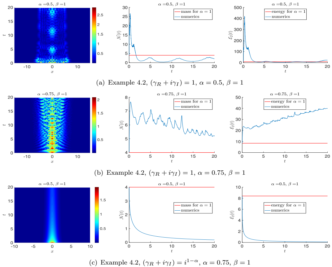
Figure 7. Evolution of the density |\psi(x, t)|^2 , mass \mathcal{N}(t) and energy \mathcal{E}_2(t) for the fractional powers \alpha = 0.5 and 0.75 for Example 4.2 (defocusing nonlinearity).
