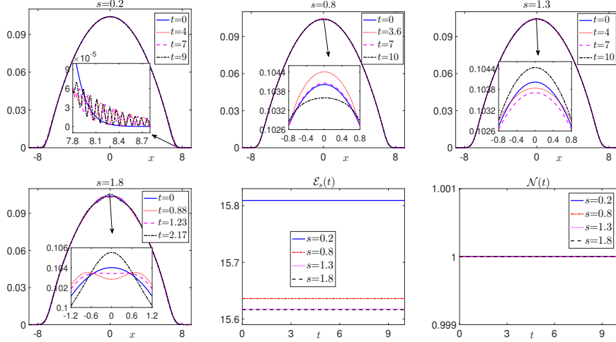
Figure 1. Density |\psi(x, t)|^2 at different times t and evolution of the mass \mathcal{N}(t) and energy \mathcal{E}_s(t) for different values of the fractional powers s for Case 1 in Example 3.1.
