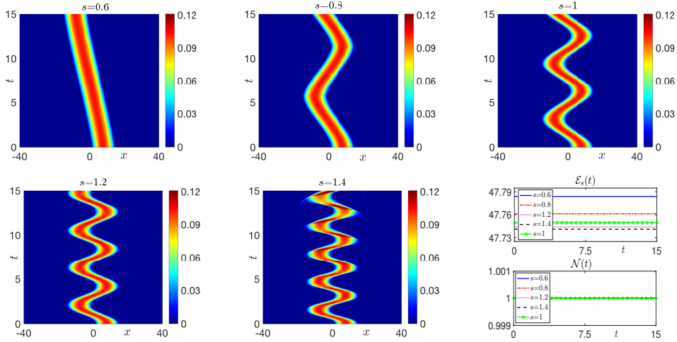
Figure 2. Evolution of the density |\psi(x, t)|^2 , mass \mathcal{N}(t) and energy \mathcal{E}_s(t) for different fractional powers s for Case 2 in Example 3.1.
