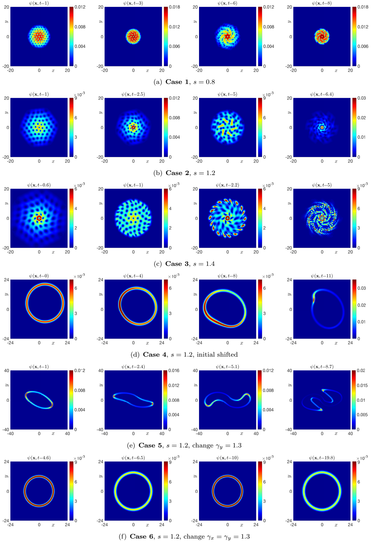
Figure 4. Initial data, contour plots of the density |\psi(\mathbf{x}, t)|^2 in Example 3.2.
