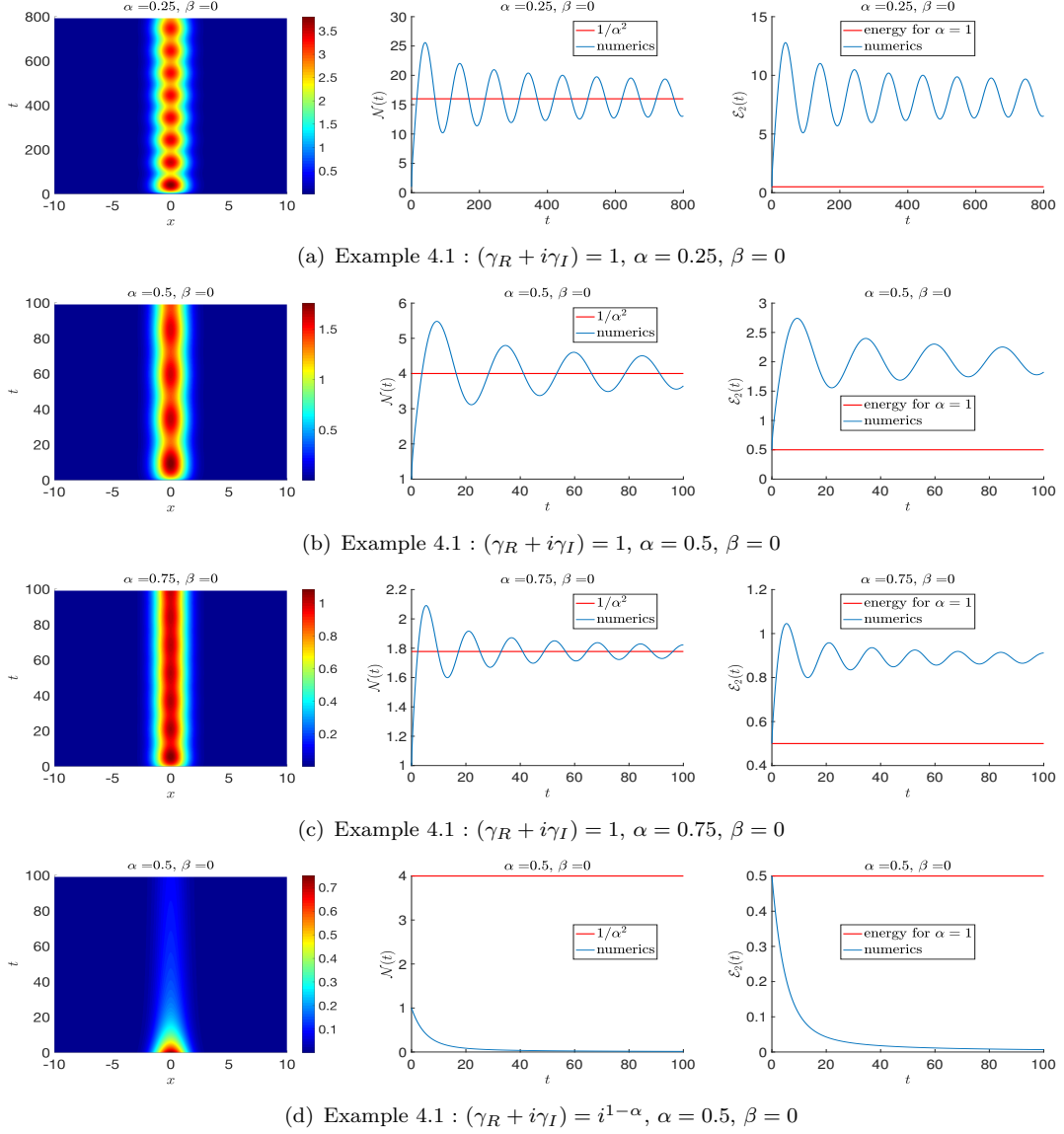
Figure 5. Evolution of the density |\psi(x,t)|^2 , mass \mathcal{N}(t) and energy \mathcal{E}_2(t) for the fractional powers \alpha = 0.25, 0.5 and 0.75 , and for the linear case \beta = 0 for Example 4.1.
