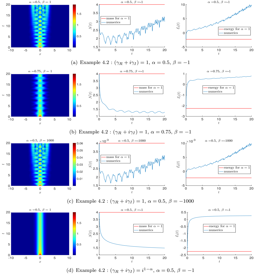
Figure 6. Evolution of the density |\psi(x, t)|^2 , mass \mathcal{N}(t) and energy \mathcal{E}_2(t) for the fractional powers \alpha = 0.5 and 0.75 for Example 4.2 (focusing nonlinearity).
