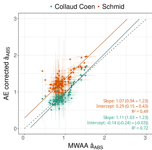
Figure 7. Scatter plot of AAE values obtained by Aethalometer corrections vs. AAE obtained from MWAA measurements. The dark-colored lines correspond to the standardized major axis linear fits and light-colored lines correspond to 1 standard deviation of the retrieved AAE data. The dashed gray line represents a 1 : 1 relationship.
