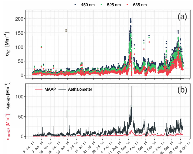
Figure 1. Time series (June–September 2014) of (a) scattering by aerosol particles measured by the nephelometer and (b) Aethalometer attenuation and MAAP absorption coefficient measurements at 637 nm during the sampling period.
