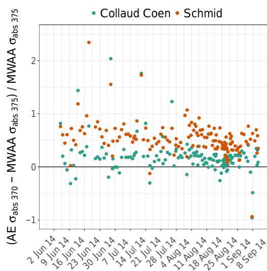
Figure 8. Overestimation of Aethalometer corrected absorption coefficients relative to MWAA at 370 nm. Values above zero are related to an overestimation of \sigma_{\text{ap}} and, below zero, to an underestimation of \sigma_{\text{ap}} at this given wavelength.
