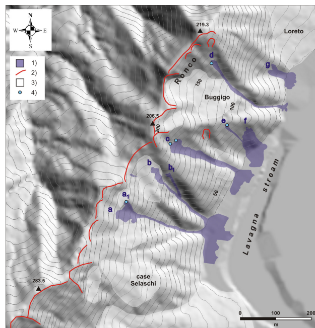
Fig. 7 - Map of shallow landslides occurred on November 10, 2014 in the Leivi slope and morphological features of ancient landslides. LEGEND: 1) shallow landslides occurred on November 10, 2014 in the Leivi slope; 2), 3) scars and deposits of ancient landslides detected by the analysis of topographic maps and aerial photographs; 4) location of sampling points
