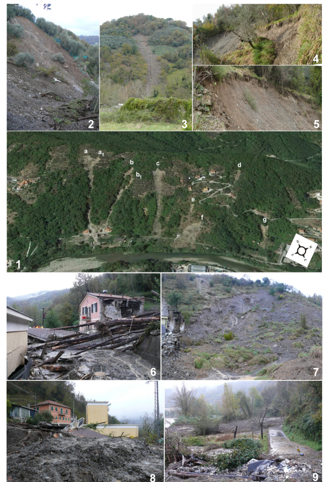
Fig. 4 - Views of the shallow landslides triggered on November 10, 2014 in the study area and related damage. 1) aerial image (from Google Earth); letters indicate the landslides; 2) detail of the source area of a large shallow landslide that gave rise to a debris flow (landslides a, a1); 3) landslide c; 4) detail of the scar of the landslide c; 5): detail of the scar of the landslide d; 6) and 8) view of the toe of the slope, where a debris flow (landslides a and a1) destroyed one building, causing two casualties; 7) landslide f; 9) damage to roads and private properties by landslide activity
