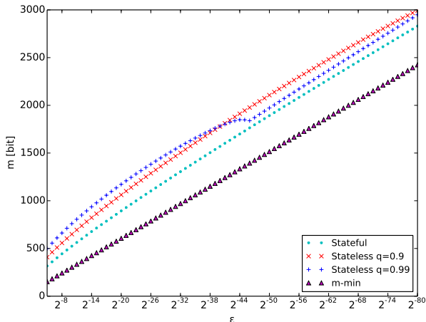
Figure 5: BF size in terms of the acceptable false positive rate \epsilon .
