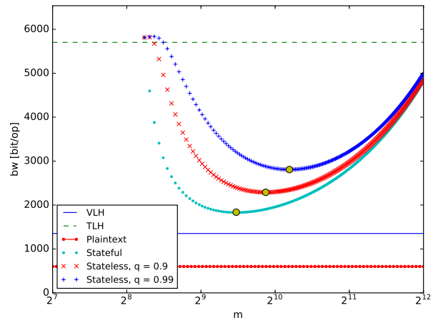
Figure 3: Estimated average network usage for each update operation in terms of the BF size m .
