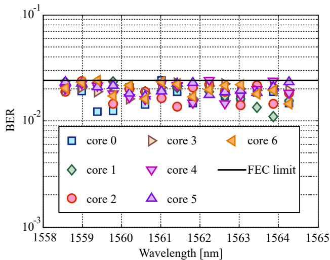
Fig. 9. BER of the 200 Gbit/s 16-QAM test channel over all 15 channels per core after a transmission distance of 720 km.
