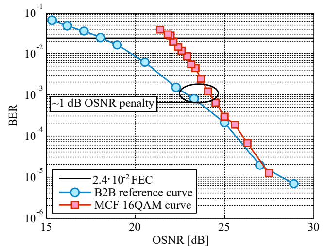
Fig. 11. BER vs. OSNR comparison between the optical B2B reference curve and the mapped points from Fig. 10
