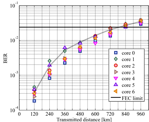
Fig. 7. Average BER measurements for the 200 Gbit/s 16-QAM test channel at 5 different wavelengths within the WDM spectrum for all cores in the MCF system. The dashed line represents the averaged BER of the 7-cores.
