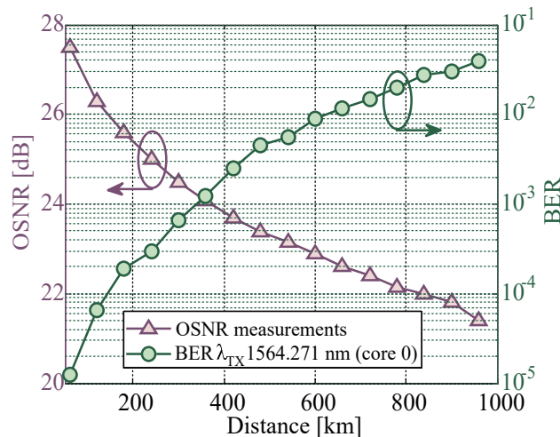
Fig. 10. OSNR (left vertical axis) and BER (right vertical axis) of a test channel at 1564.27 nm for the MCF transmission system.
