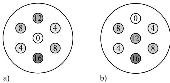
Fig. 6. Relative delay lines in meters with respect to a given core to de-correlate signals between optical waveguides: a) with respect to the middle core, and b) with respect to one of the outer cores.
