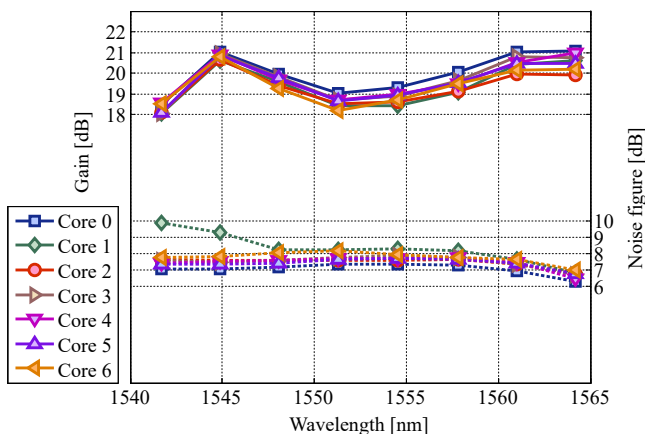
Fig. 5. Approximate gain spectrum and noise figure of the 7-core MC-EYDFA for an MMPD current of 2 A. The gain spectrum takes into account the average insertion loss of one integrated multicore isolator.
