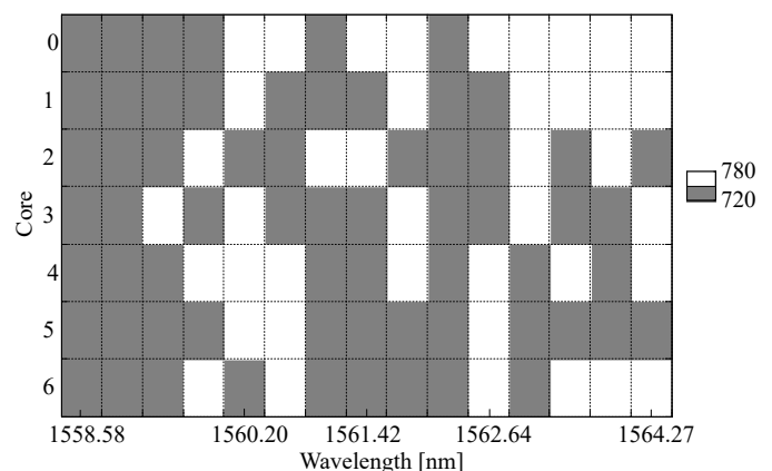
Fig. 8. Maximum achievable distance of the 200 Gbit/s test channel over all 15 channels per core before crossing the assumed FEC threshold of 2.4 \cdot 10^{-2} .
