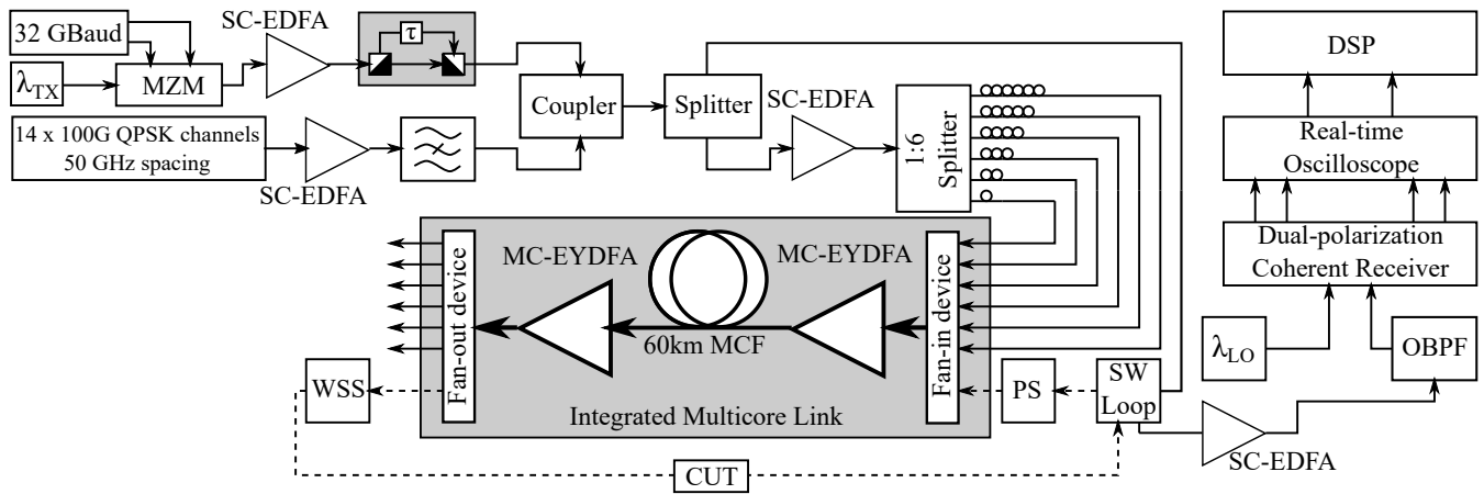
Fig. 4. Experimental setup of the multicore fiber system. SW Loop refers to the optical switches used to let the signal in and out of the recirculating loop. This setup analyzes the transmission performance of a given core of the MCF, while the remaining cores act as sources of inter-core crosstalk.
