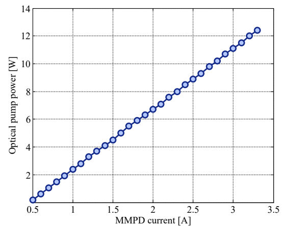
Fig. 3. Relation between the diode current and the optical pump power produced by the MMPD in the amplifiers.
