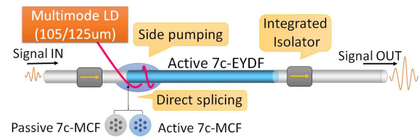
Fig. 2. Schematic diagram of the internal structure of a MC-EYDFA. The position of the integrated isolator in the MC-EYDFA depends on the role of the amplifier in the system. A pre-amplifier has the isolator at the input of the MC-EYDFA, whereas a post-amplifier has it placed at the output.
