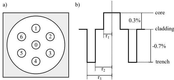
Fig. 1. a) Hexagonal waveguide layout and core identifiers of the 7-core MCF used in the experiments. b) Refractive index profile of the 7-core MCF.
