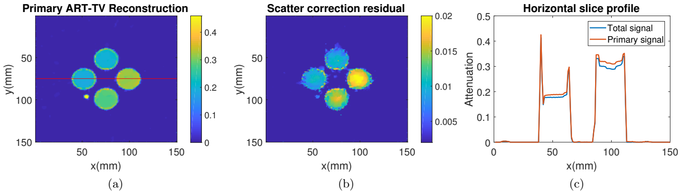
Figure 6: (a) The slice reconstruction of the primary attenuation A_p(\vec{r}, E) . The overlapping red line shows the horizontal line corresponding to the profile plotted in (c). In the latter the blue line is the result of the total attenuation A_t(\vec{r}, E) , while the red line is the result of the primary attenuation A_p(\vec{r}, E) obtained by the subtraction of the scattering contribution from the total signal. The residual of the two reconstructions (namely of A_p(\vec{r}, E) and A_t(\vec{r}, E) ) is displayed in (b).
