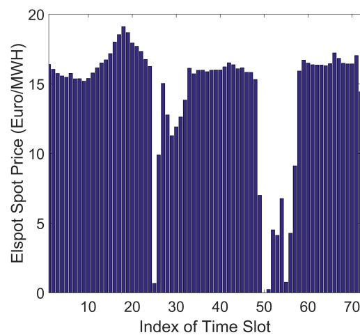
Figure 6. Electricity prices in 72 time slots. For each slot, it presents one hour.
