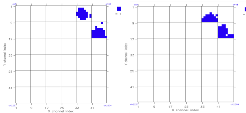
Figure 6: Each is one of frames response from beam test. It takes 6msec to take a frame data. UBAT has 6 \times 6 MAPMTs originally but mini UBAT has only 2 MAPMTs. Its locations are (1,5) and (2,6). Blue color is response for any particles and white color is no response.
