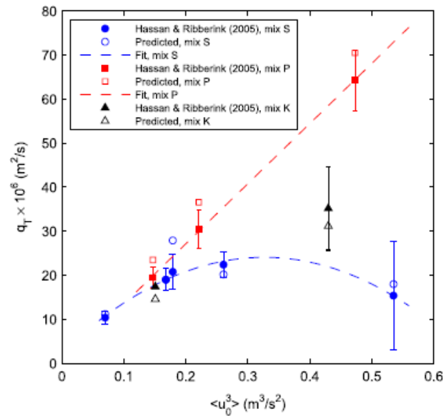
Figure 3. Measured and predicted net sediment transport rates versus the third moment of the free stream velocities for the non-uniform sand cases from HR. The experimental error bars for each case are also shown. The dashed lines are curve fits to the experimental data from mix S and P. This figure is reprinted from Caliskan and Fuhrman (2017) with permission from Elsevier.
