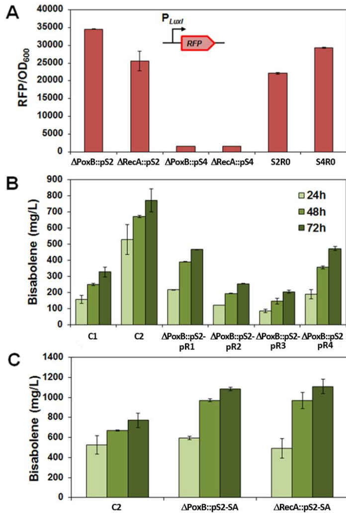
Figure 6. Bisabolene production of genome integrated QS strains. (A) Two genome locations were chosen: recA and poxB to insert pS2 and pS4 QS sensor variants. RFP reporter gene driven by P_{luxI} promoter was used for characterization. The response signal from QS-integration strains are: \Delta PoxB::pS2 (JBEI-7581), \Delta RecA::pS2 (JBEI-7582), \Delta PoxB::pS4 (JBEI-7583), \Delta RecA::pS4 (JBEI-7584), and their cognate plasmid-borne QS strains: S2R0, and S4R0. (B) Four production plasmids (pR1 to pR4) were transformed into \Delta PoxB::pS2 strain, and the bisabolene productions from these strains were measured and compared to control strain C1 and C2. C1 consists of plasmids pS0 and pC1, C2 consists of plasmids pS0 and pC2. pC1 contains P_{lacUV} -driven MevT-MBIS operon and P_{trc} -driven BIS gene, pC2 contains P_{lacUV} -driven MevT operon, P_{trc} -driven MBIS operon and P_{trc} -driven Bis gene. (C) Bisabolene production was measured in QS strains \Delta PoxB::pS2 and \Delta RecA::pS2 . Both strains ( \Delta PoxB::pS2 -SA and \Delta RecA::pS2 -SA) contains plasmids pSMevT (pJBEI-7554) and pAMBIS-Bis (pJBEI-7555).
