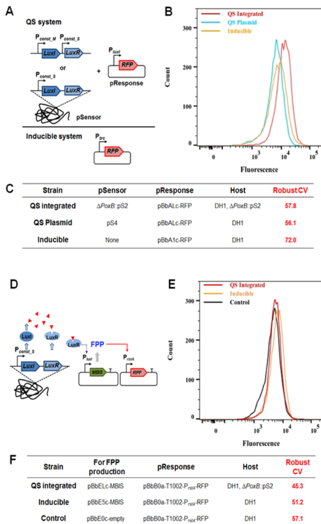
Figure 7. Analysis of the population distribution of protein expression and producing cell using flow cytometry. The fluorescence intensity of individual cells was measured by flow cytometry at 10-hr post-induction. (A) Schematics of the QS systems and IPTG-inducible system activating RFP expression. (B) RFP Fluorescence intensity and distribution spread of QS-integrated system, QS-plasmid borne system and inducible system. (C) Description of the strains and robust coefficient of variation (rCV) (D) Schematics of QS system activating the FPP biosynthesis pathway and FPP molecule activating RFP expression. (E) Fluorescence intensity and distribution spread of the QS-integrated, inducible and control systems. The QS and inducible systems contain FPP producing pathway and RFP. (F) Description of the strains and rCV.
