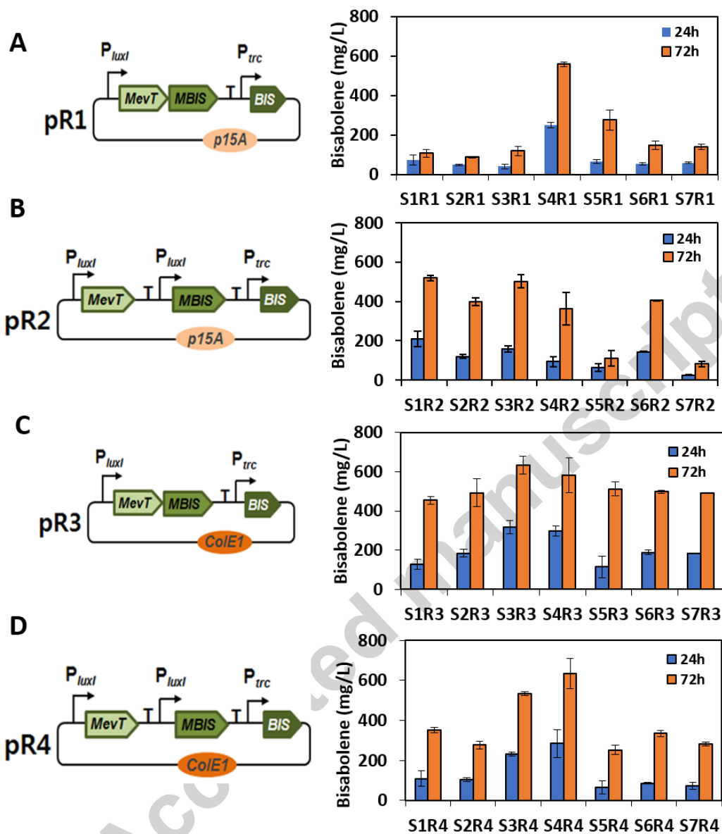
Figure 5. Optimization of bisabolene production by a combinatorial approach using 7 pSensor variants and 4 production plasmid variants (pResponse). Left: Plasmid architecture of each pResponse variants. Right: Bisabolene titer after 24 and 72 hours. (A) Titer from pR1 production plasmid; (B) Titer using pR2 production plasmid; (C) Titer using pR3 production plasmid; (D) Titer using pR4 production plasmid.
