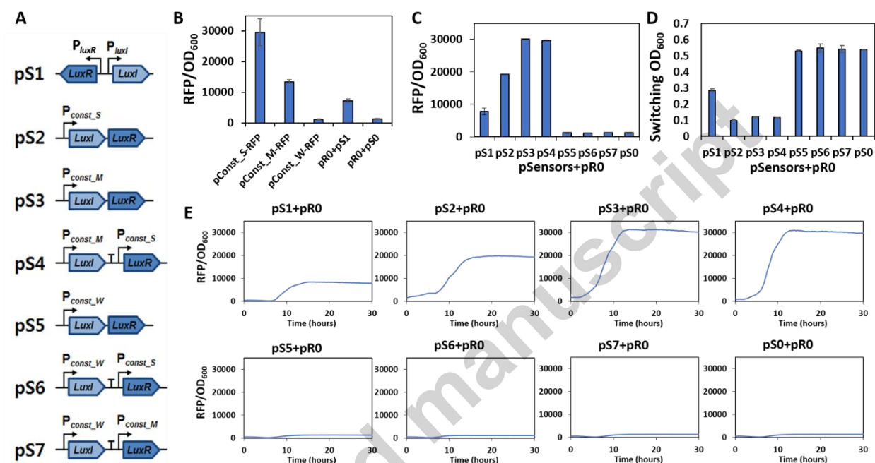
Figure 4. Construction and characterization of QS sensor variants. pR0 plasmid containing RFP reporter gene was co-transformed with each pSensor variant during the characterization. (A) Schematics of pSensor variants with different constitutive promoters. (B) Comparison of promoter strength between constitutive promoters P_{const\_S} , P_{const\_M} , P_{const\_W} and P_{luxI} promoter in S0R0 and S1R0 strains. (C) End point RFP activation signal among pSensor variants. (D) Cell density ( OD_{600} ) of the time that RFP was activated among seven pSensor variants. (E) Time-course RFP activation signal among pSensor variants. The P_{luxR} promoter region is poorly defined and thus not included in the promoter strength analysis.
