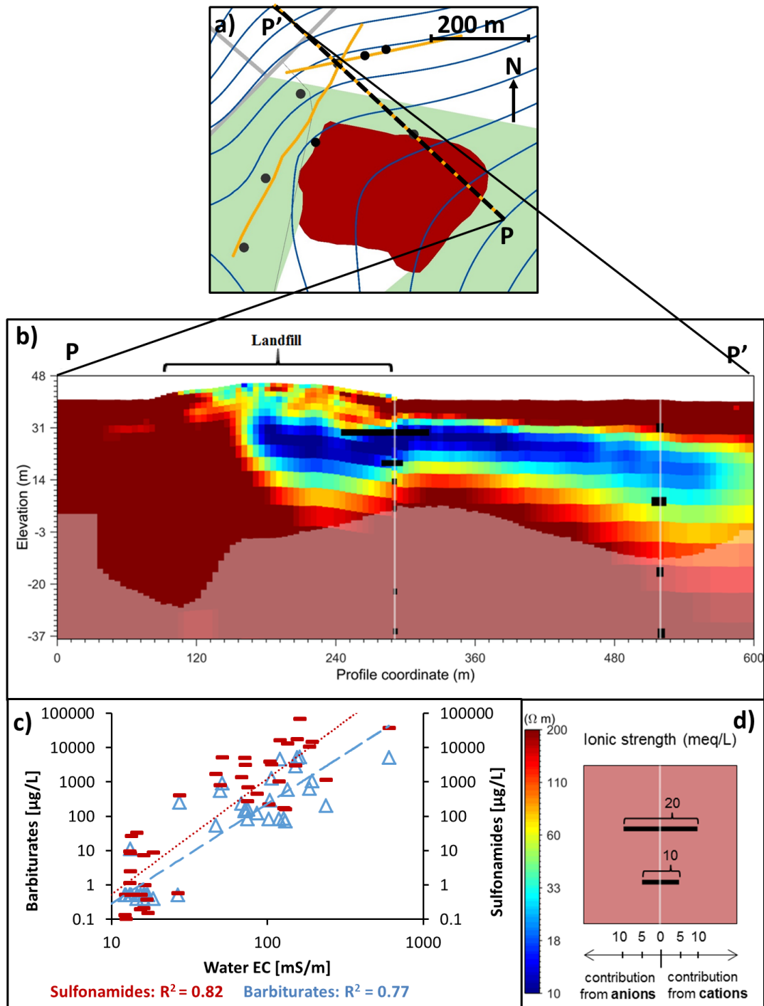
Figure 6: Locations of the DCIP profiles (orange lines) and multilevel sampling wells (black dots) are shown in a) for the landfill site. The bulk electrical resistivity and the ionic strength from water samples (black bars) are shown in b), legend shown in d), for the profile parallel to the groundwater flow direction indicated by the black line in a). The correlation between the water electrical conductivity (EC) and the concentration of sulfonamides and barbiturates are shown in a log-log plot in c). Modified figure from Balbarini et al (II) and Maurya et al (IV).
