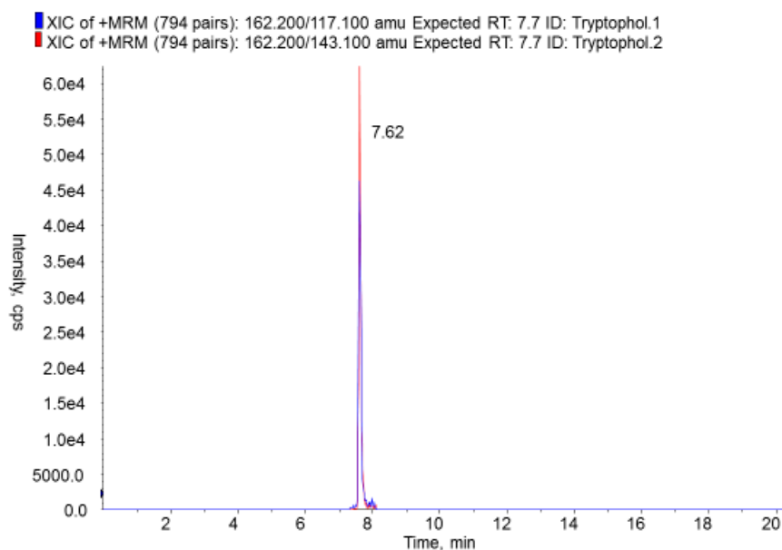
Figure 1. Overlay of XICs on tryptophol.
