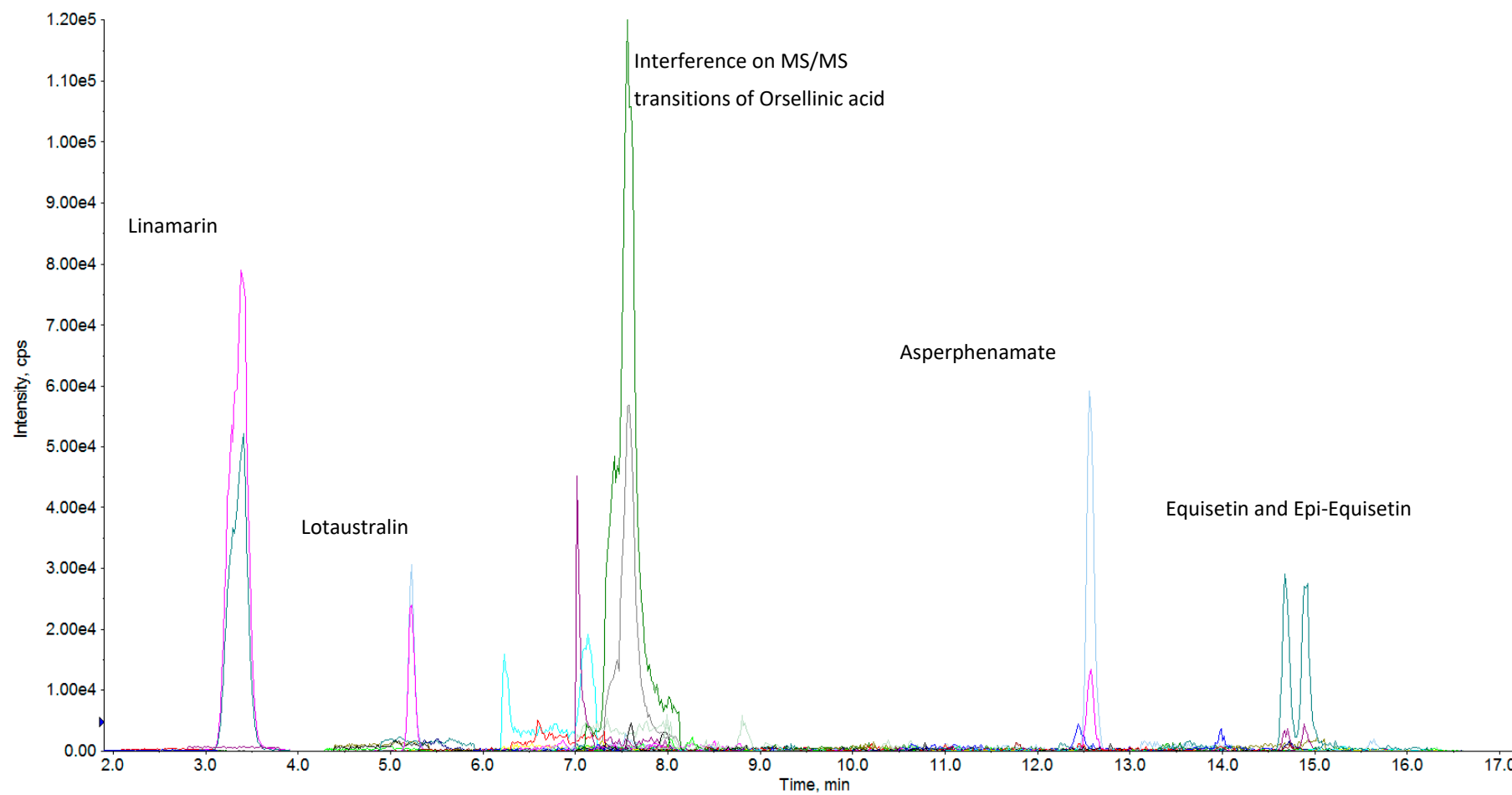
Figure 2. Overlaid ESI (-) MRM-chromatogram (sum of all XICs) in a representative sample.
