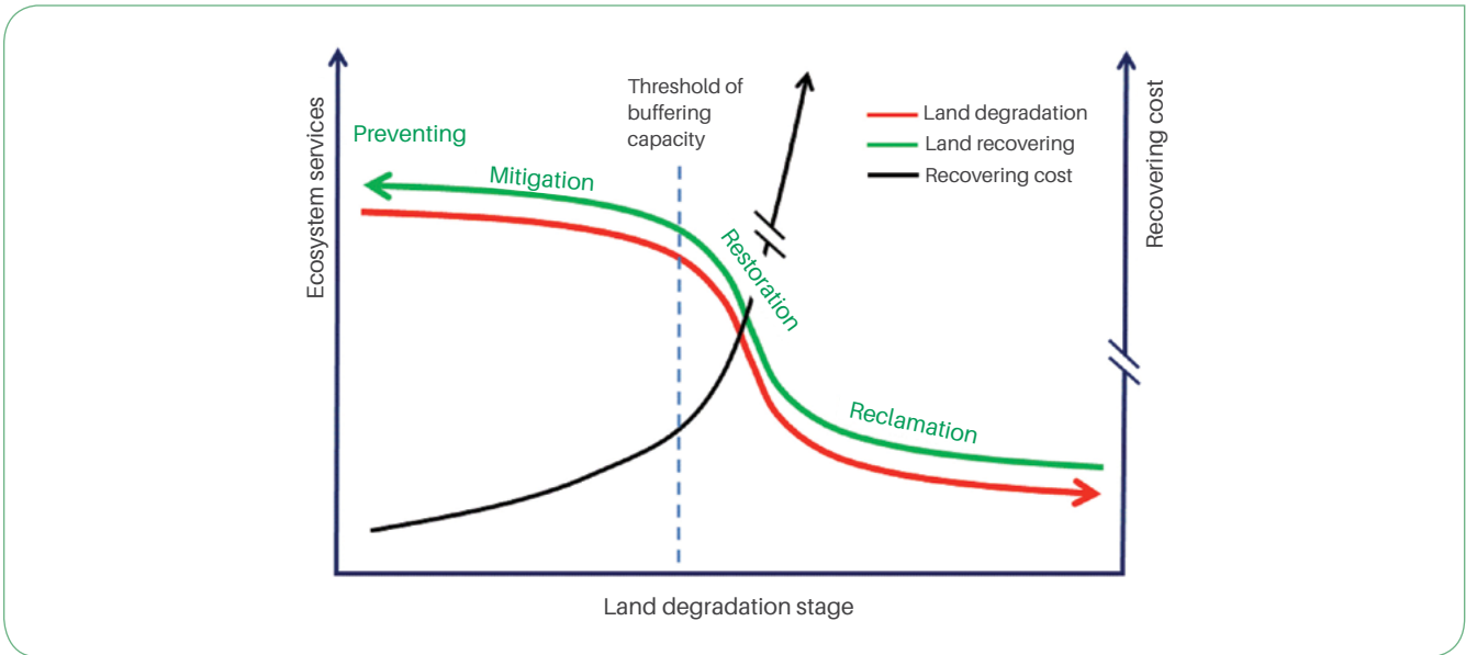
Figure 4.2 Stages of land degradation (red line) and the relevant management strategies at the various stages of this process and the associated cost. The reversal (green line) often takes much longer than the degradation process.
