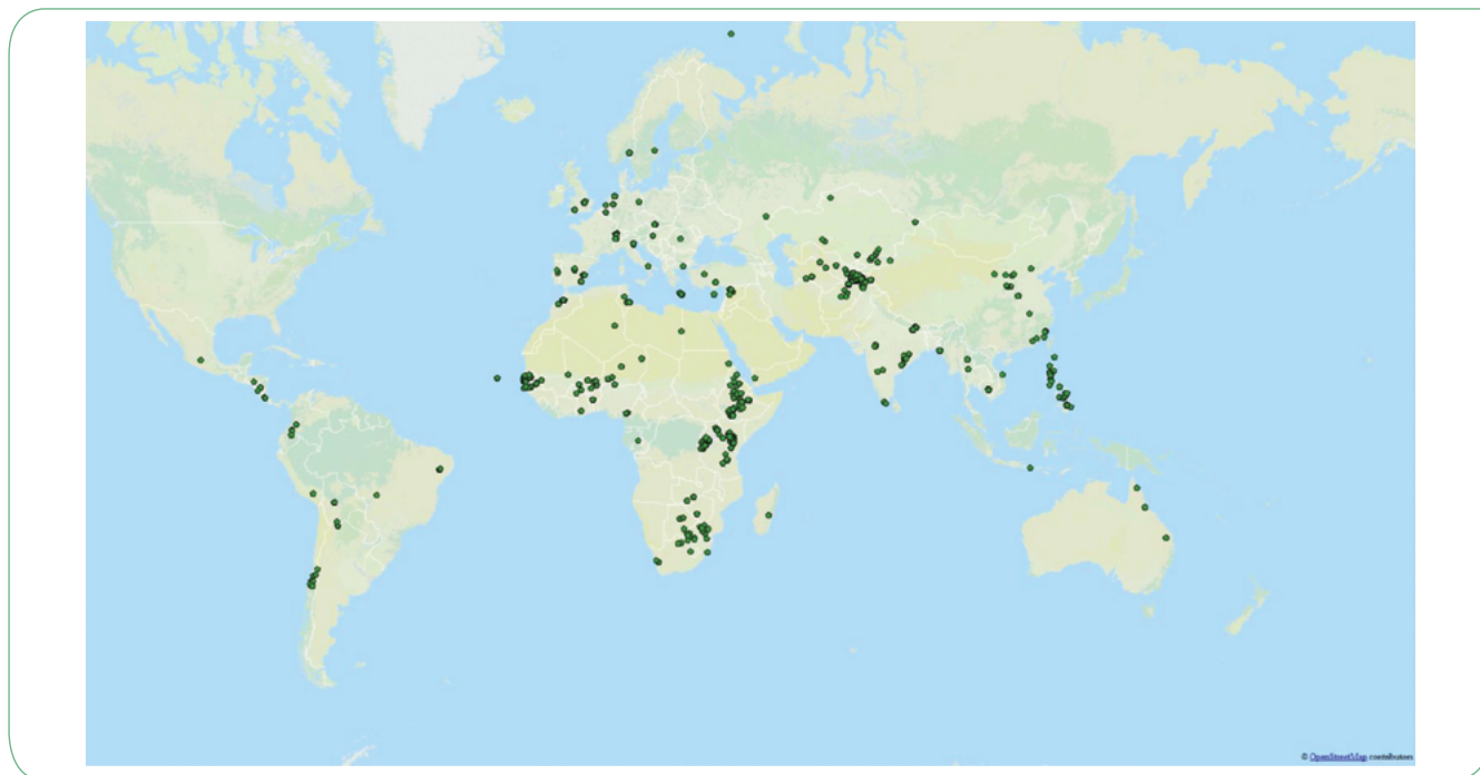
Figure 4.4 Location of documented sustainable land management (SLM) technologies with claimed land conservation outcomes in the WOCAT database.
