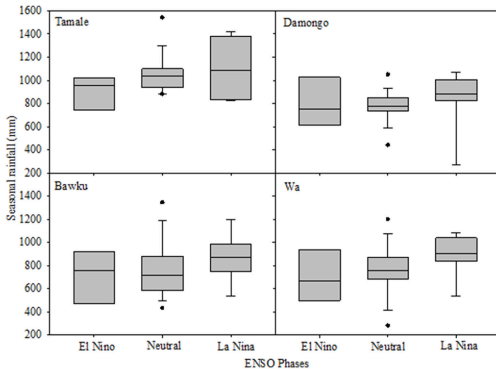
FIGURE 1 | Box plots of seasonal rainfall distributions according to the ENSO phases (1980–2009) for 4 sites in northern Ghana. Each box in the graph shows the distribution of rainfall for a specific ENSO phase. The boundary of the box closest to zero indicates the 25th percentile, a line within the box marks the median, and the upper boundary of the box indicates the 75th percentile. Whiskers above and below the box indicate the 95th and 5th percentiles.
