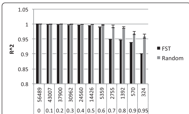
Fig. 6 Average accuracy ( R^2 ) and standard deviation (error bars) of ADMIXTURE -based estimation of individual ancestries using: i) SNP panels selected according to increasing F_{ST} thresholds compared with; ii) same number of randomly selected markers. The accuracy was estimated by correlating the ancestry estimates from the various subsets with that obtained using the entire marker data
