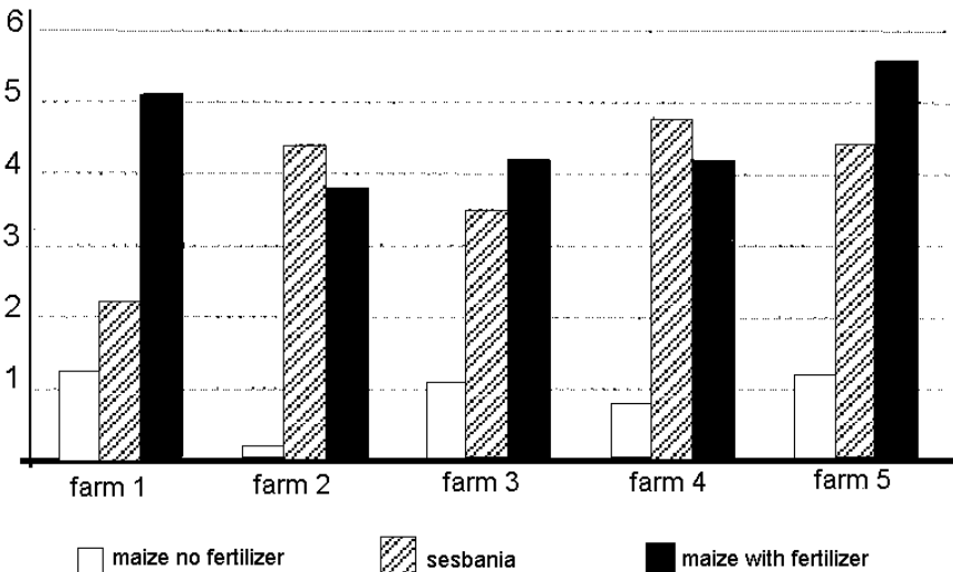
Figure 20: Maize yields in tons per ha on 5 farms over a 3-year period (1993 -96), with or without fertilizer, and following a 2-year sesbania fallow. Fertilizer treatment: 112 kg N, 40 kg P 2 O 5 , 20 kg K 2 O per ha. (Source: Kwesiga & Beniest, 1998)
