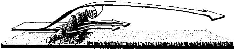
Figure 14: The shelterbelt should allow some wind to pass through, to reduce turbulence. Note that there is also turbulence behind a permeable windbreak, but that it stays above the trees. Lower down the wind speed is greatly reduced and the crops are protected.
