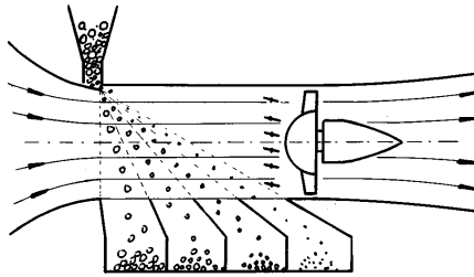
Figure 3.5.5 Vanneuse
