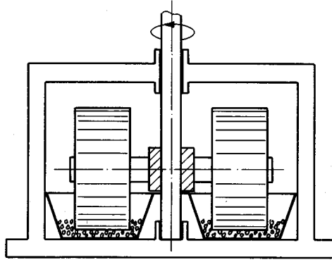
Figure 3.6.9 Kollergang
