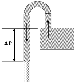
Figure 3.2.8 Siphon \Delta P = pression hydrostatique
