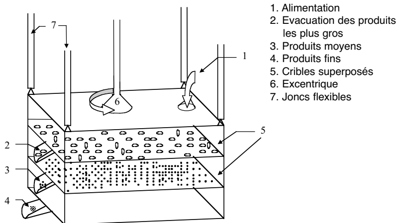
Figure 6.2.2 Planschister
