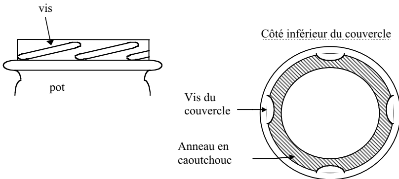
Figure 3.7.9 Couvercle "Twist-off"
