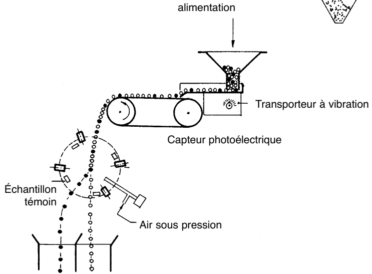
Figure 3.5.7 Classification pneumatique
