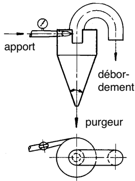
Figure 3.5.3 Hydrocyclone
