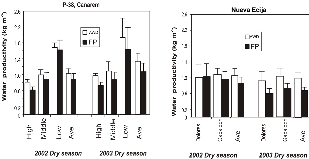
Fig. 10. Average water productivity (kg m -3 ) at the pilot sites in Tarlac (left) and Nueva Ecija (right) for 2002 and 2003 DS.
