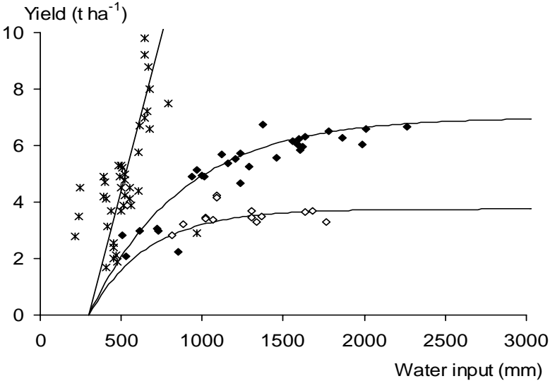
Fig. 3. Yield versus water input. Data from field experiments in India in 1976 and 1978 (◇, Jha et al 1981), in India in 1981-1982 (◆, Tripathi et al 1986), and in Japan (*, Anbumozhi et al., 1998). The curved lines are fitted production functions of the shape [yield = a*(1 - e (b*(water input - c)) )]. (Source: Bouman and Tuong, 2001).
