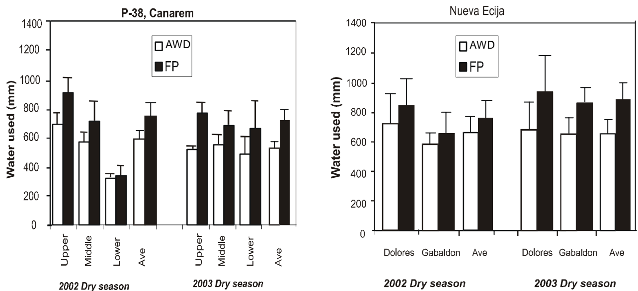
Fig. 8. Total water used (mm) at AWD and FP plots in Tarlac (left) and Nueva Ecija (right) for 2002 and 2003 dry seasons.
