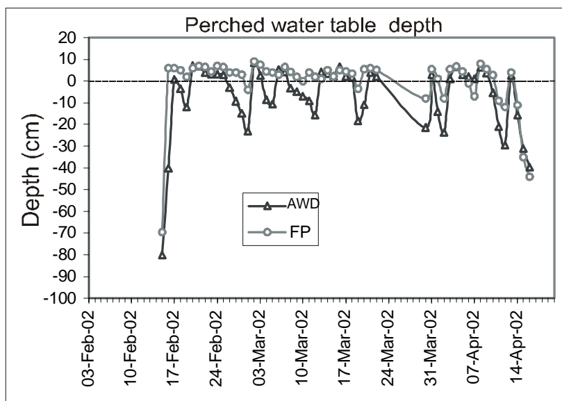
Fig. 6. Typical perched water table depth in Gabaldon in dry season 2002.
