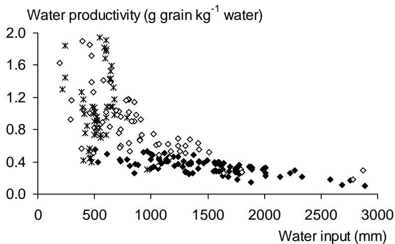
Fig. 2. Water productivity versus water input. \blacklozenge are data from Indian field experiments ( N = 99 ), \diamond are data from Philippine field experiments ( N = 61 ), \times are data from Japanese and Philippine pot experiments ( N = 48 ). (Source: Bouman and Tuong, 2001.)
