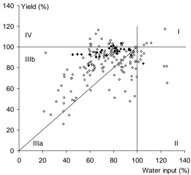
Fig. 1. Relative yield versus relative water input under saturated soil culture (SSC) (black diamonds) and alternate wetting and drying (AWD) (open diamonds) conditions. The relative yield and water inputs are calculated as the yield and water input of the SSC and AWD treatments as percentage of the yield and water input of the checks (continuous flooding), respectively. Data from Indian and Philippine field experiments. (Source: Bouman and Tuong, 2001.)
