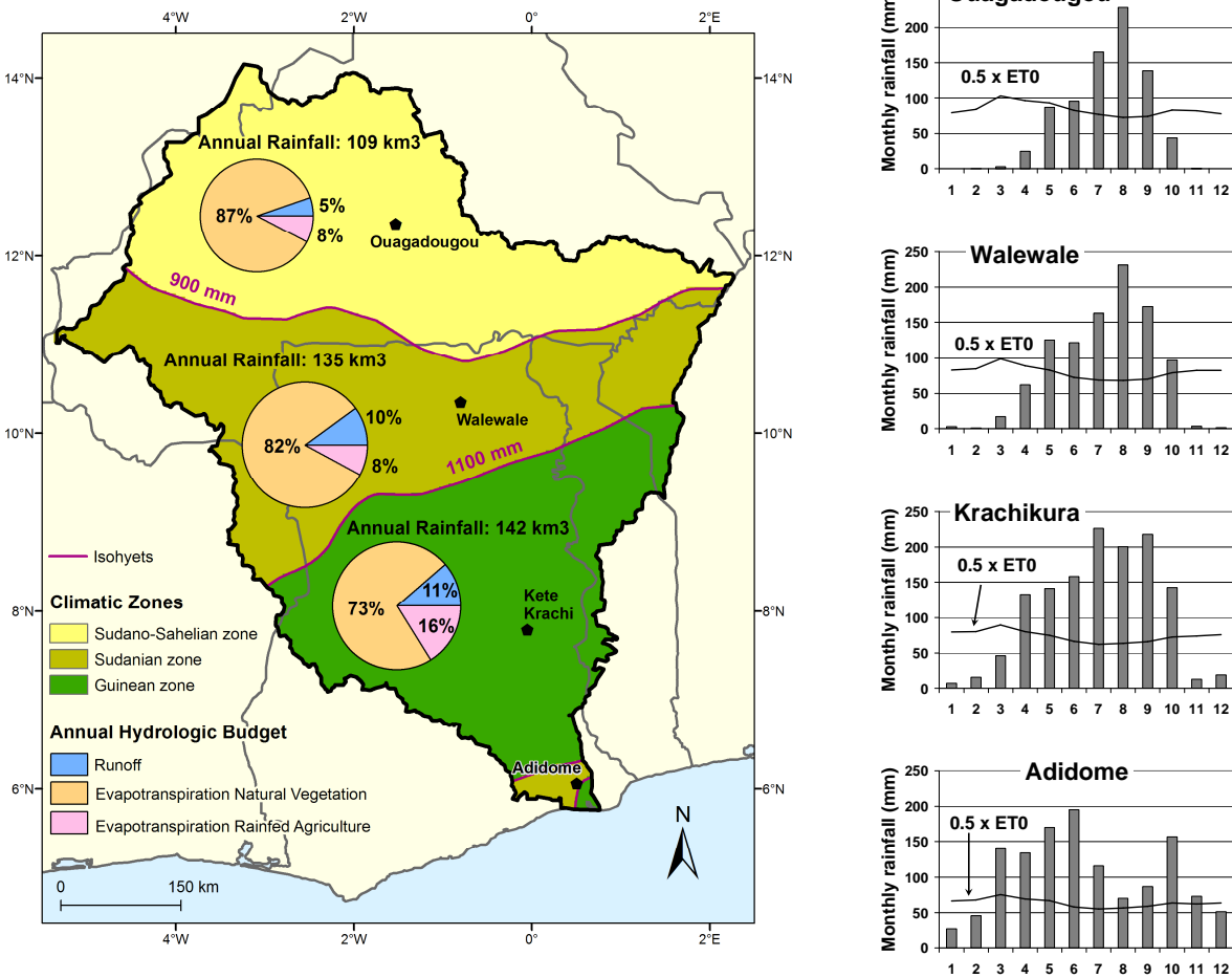
Figure 6. The agro ecological zones with a summary of the water account in the Volta basin, and the distribution of rainfall in four stations along the south-north gradient. ET 0 is the reference (or potential) evapotranspiration. The intersection of the 0.5 ET 0 line with the rainfall distribution indicates the length of the growing season (map by BFP Volta with data from CRU) (De Condappa et al. 2008).
