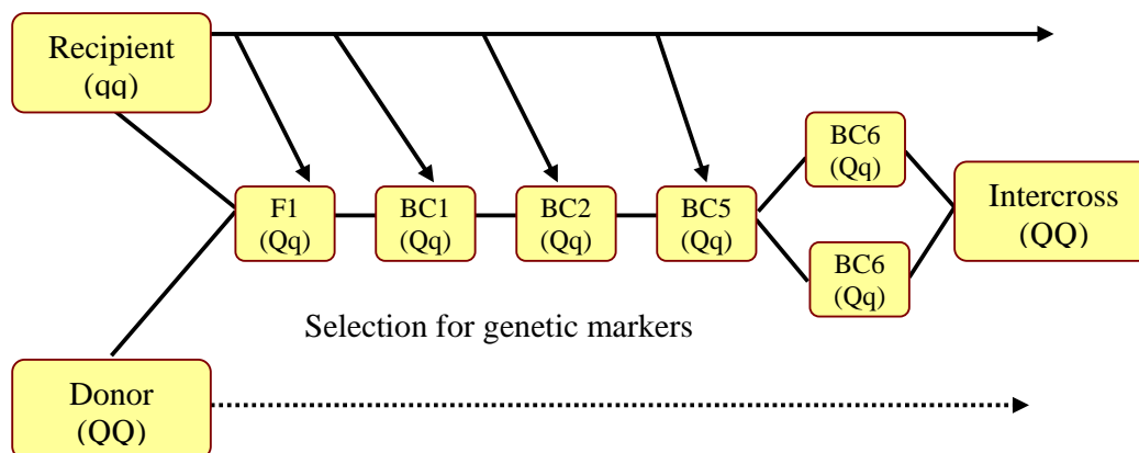
Figure 5. An introgression breeding scheme with MAI.
