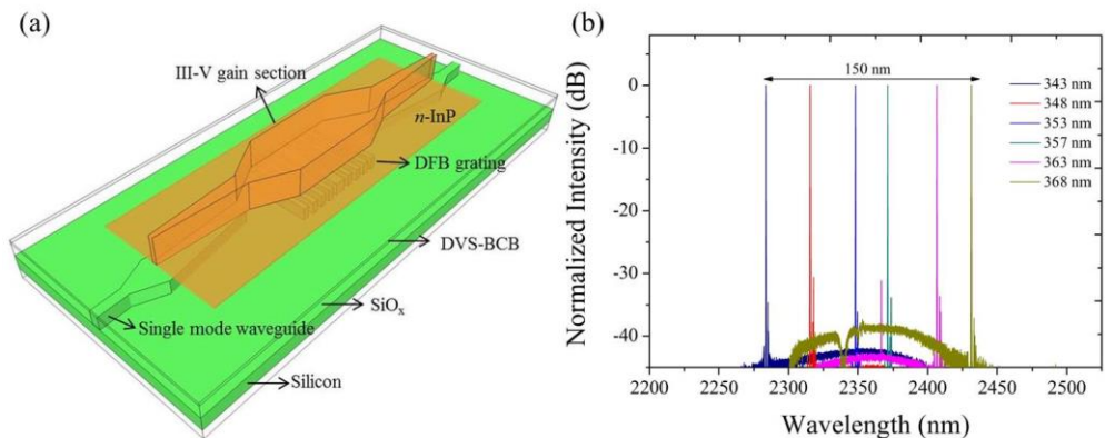
Fig. 1. (a) Schematic of the heterogeneously integrated DFB laser; (b) normalized emission spectra of six DFB lasers with different grating period in an array.
