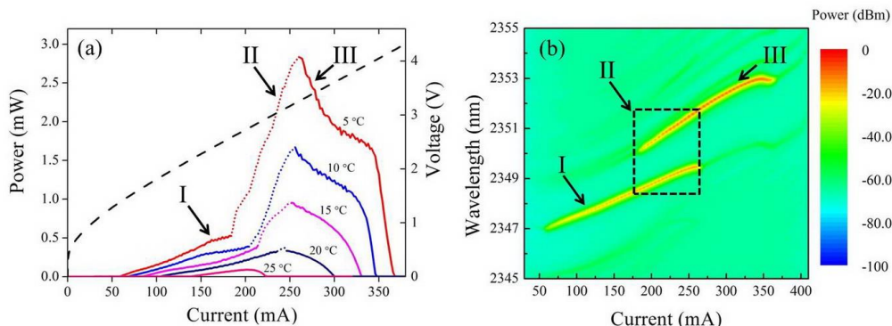
Fig. 2. (a) P-I-V curve of the DFB laser with grating period of 353 nm; (b) 2-D optical spectra of the device as a function of the injection current at 5 °C.
